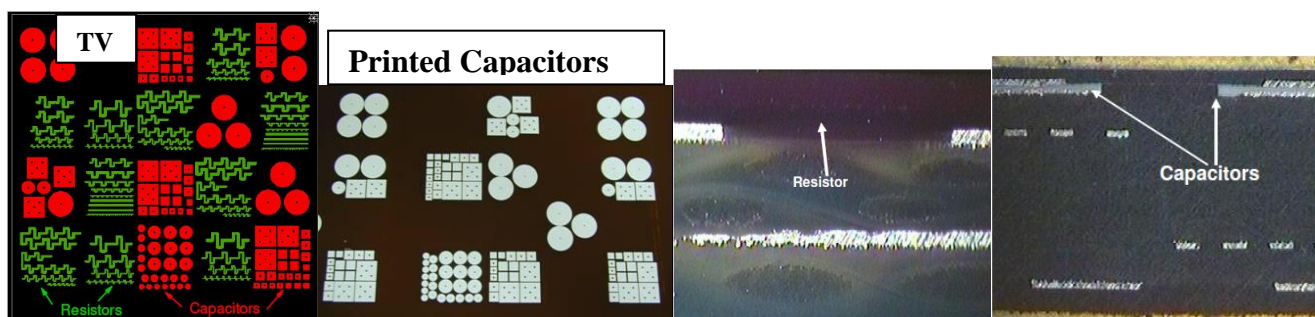
Figure 4A: Representative test vehicle (TV) and corresponding cross-section view of screen printed embedded capacitors and resistors (Collaboration: Georgia Tech PRC and Nokia)
