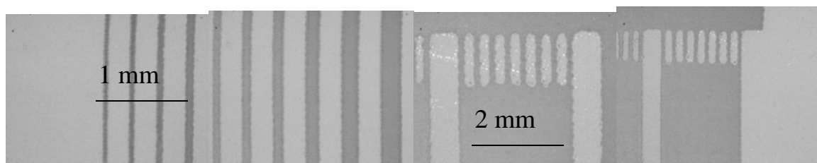
Figure 5 : Printed resistors
