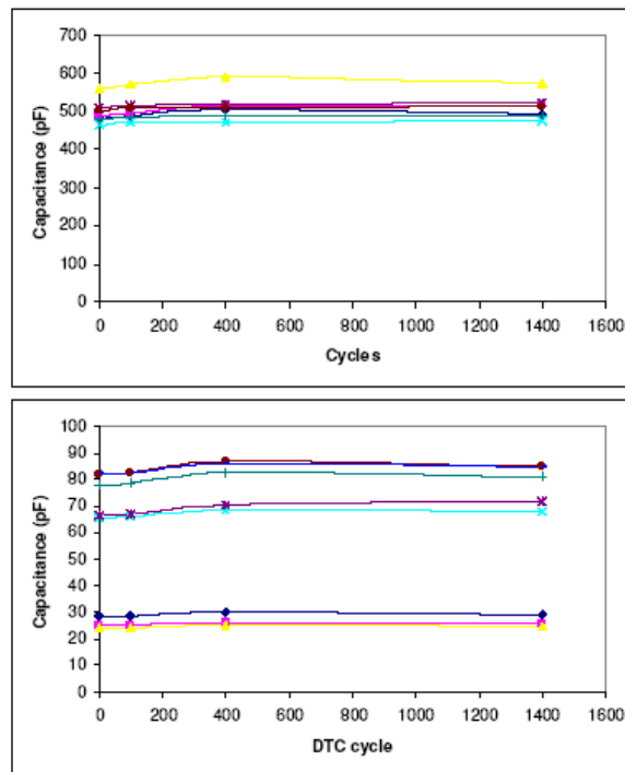
Figure 12: Change in capacitance after IR reflow (assembly) pre-conditioning (3X, 245°C) and thermal shock up to 1400 cycles (-55C-125C) for large, medium and small capacitors for embedded capacitors
