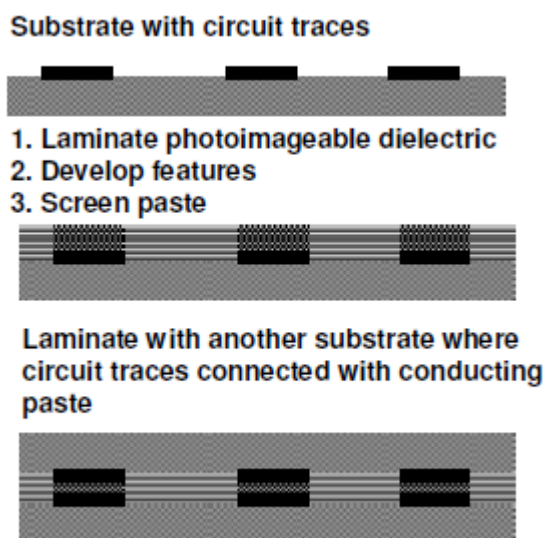
Figure7 : Schematic presentation for making screen printable Interconnects
