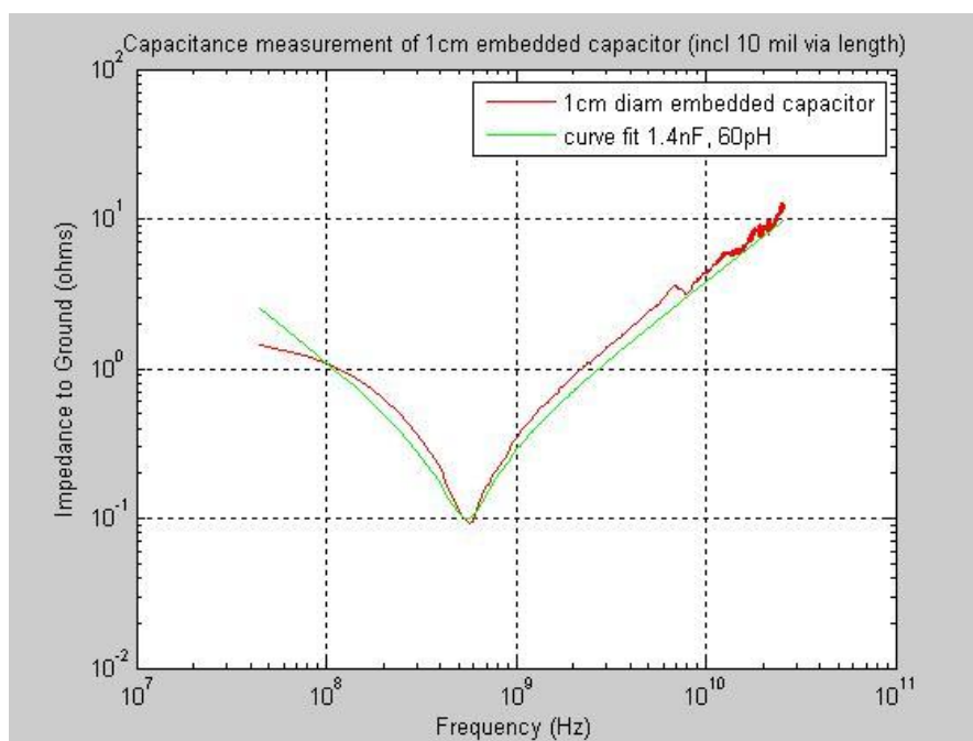
Figure 4B: Impedance profile of Capacitors
