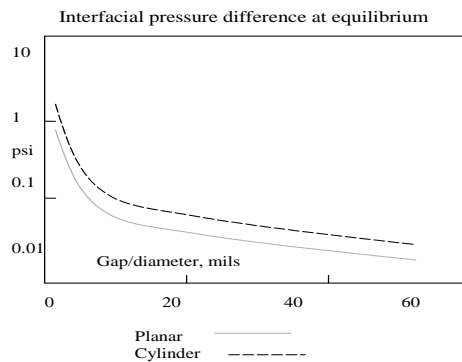
Figure 2: Relationship between gap size and capillary force for water on glass
