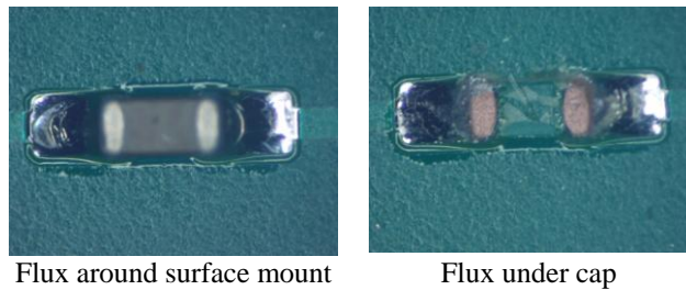
Figure 1: Flux residues around and under the component
