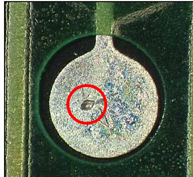
Witness mark of a 40 ° razor on a flat lead-free soldered test pad, no-clean process
