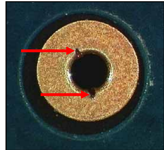
Witness mark of a 90 ° razor on an OSP via, unpasted, no-clean process.
