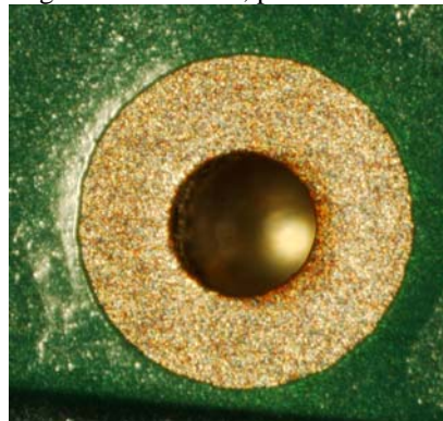
Figure 3 –OSP via (backside of pasted via).
