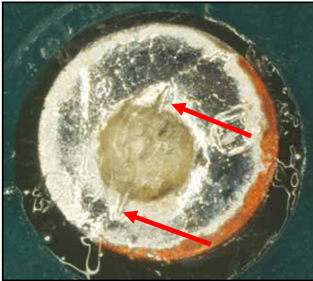
Witness mark of a 150° razor sharp tip on lead-free pasted via, no-clean process
