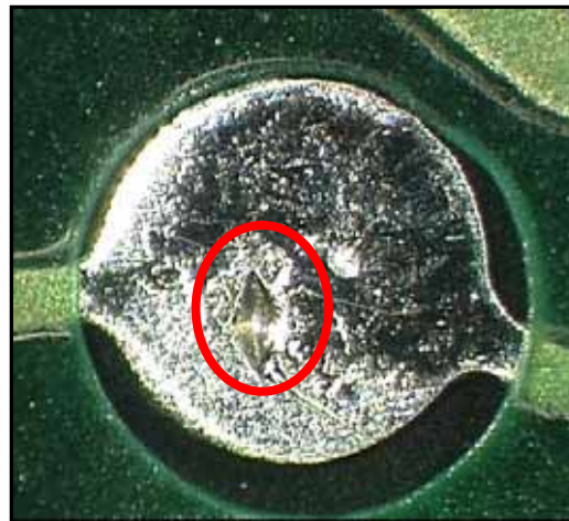
Witness mark of a 90 ° razor on a lead-free pasted test pad, no-clean process.
