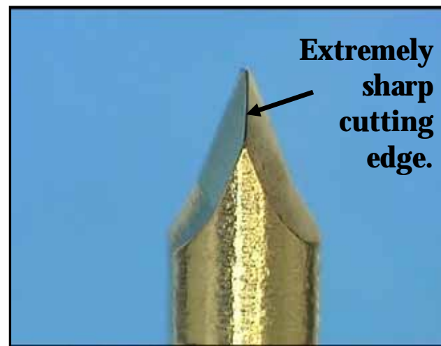
Side view with 45° secondary angle.
