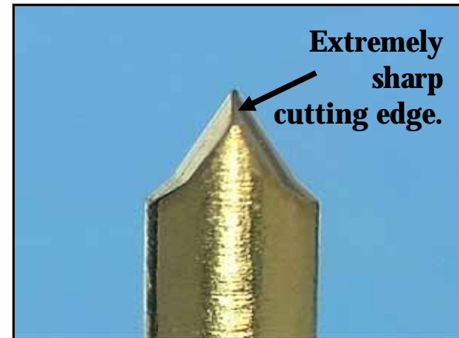
Side view with 60° secondary angle.
