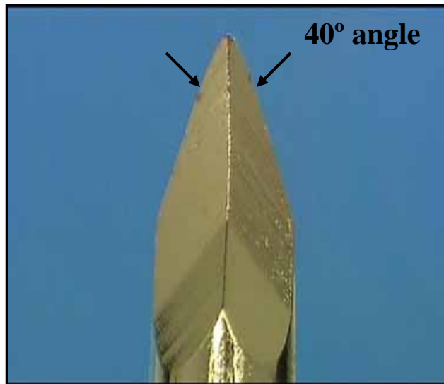
Front view primary angle.
