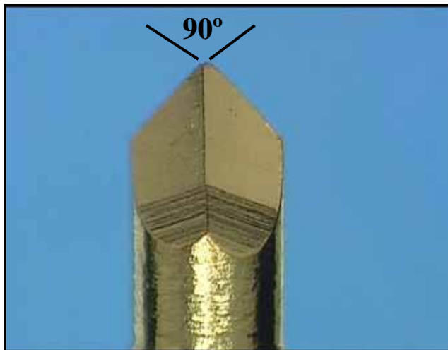
Front view primary angle.
