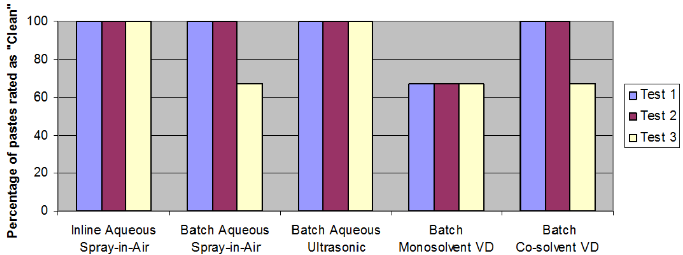
Cleaning results for Sn/Pb solder by process
