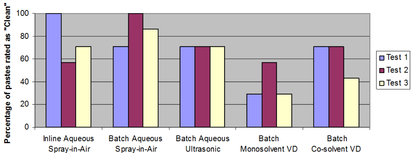
Cleaning results for Pb-free solder by process
