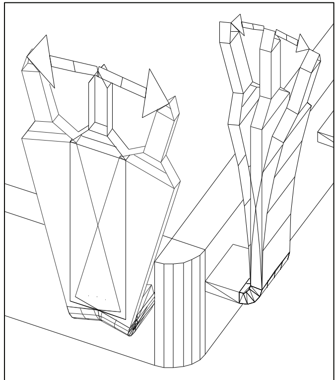
Figure 25 –The figure tries to illustrate the difference in the bending resistance of the leads. If we try to bend the lead “across flats”, as with the lead at the right hand side of the figure, we can feel that the lead is fairly flexible. By contrast, if we try to bend the lead “across edge”, as with the lead at the left hand side of the figure, we will notice that the lead behaves as a very stiff lead or very stiff spring. That is if we want to have the same amount of deflection in both cases. The result is that trying to get the same amount of deflection at the left lead, will induce very high stresses at the base of the lead and may create micro-cracks in the plastic housing of the package, allowing moisture to migrate to the chip and shorten its operating life.
