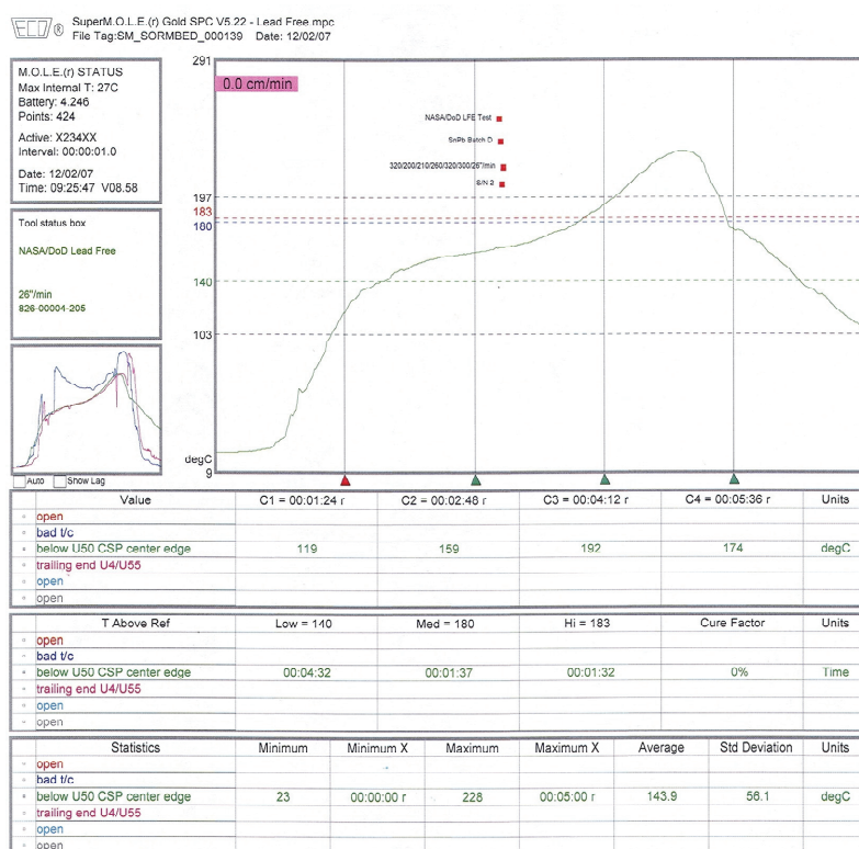
Figure 2. Reflow Profile for SnPb Solder Paste
