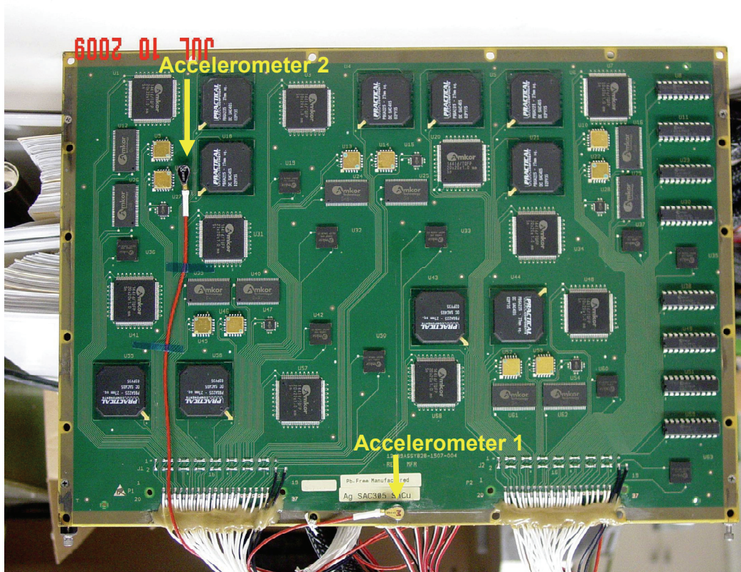
Figure 1. NASA-DoD Test Vehicle
