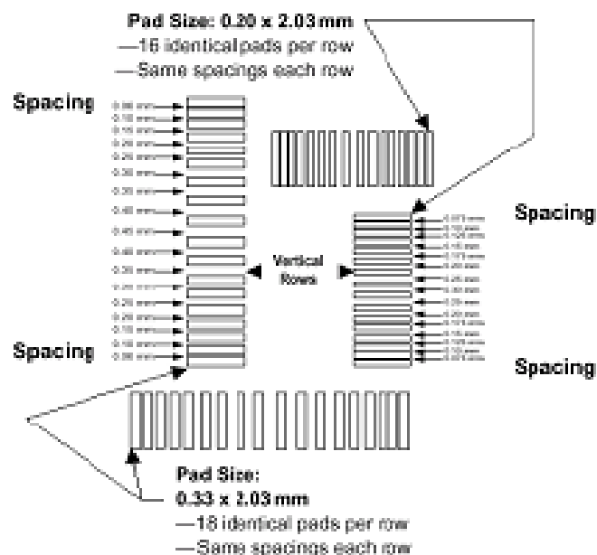
IPC-A-20 stencil pattern
