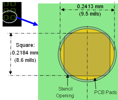
Figure 8: Close up of stencil opening design for Nano & E-Fab.
