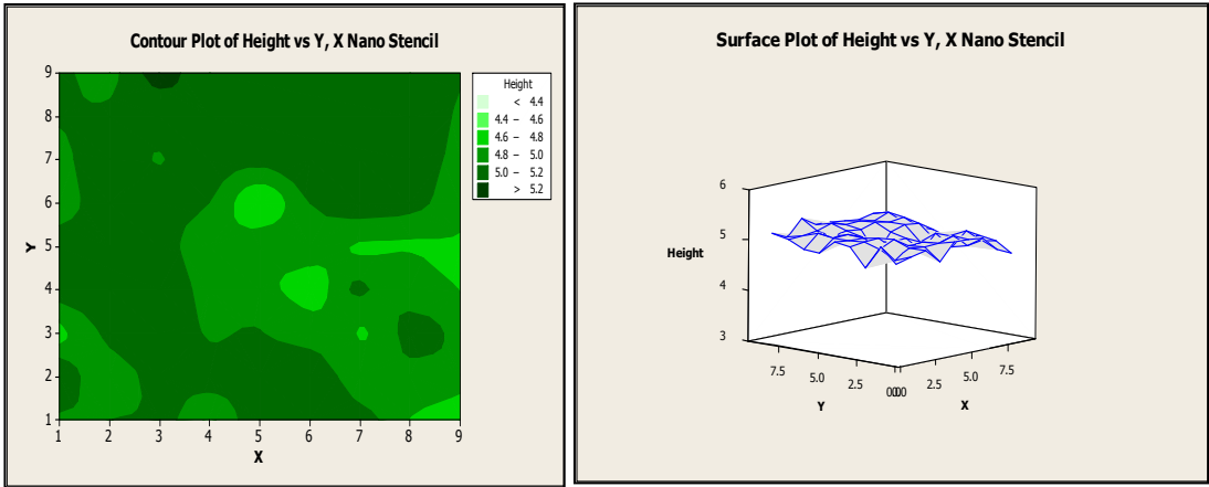
Figure 14: Nano coated stencil, paste height distributions along the 0.4 mm pitch CSP (in mils), lot size: 240 PCA.
