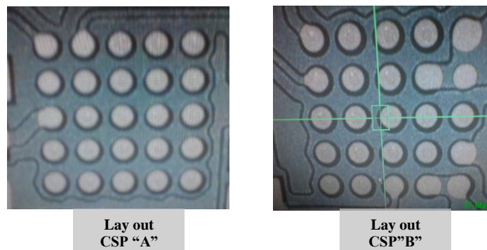
Figure 31: Close up of the pad land pattern for two 0.4 mm pitch CSP's.
