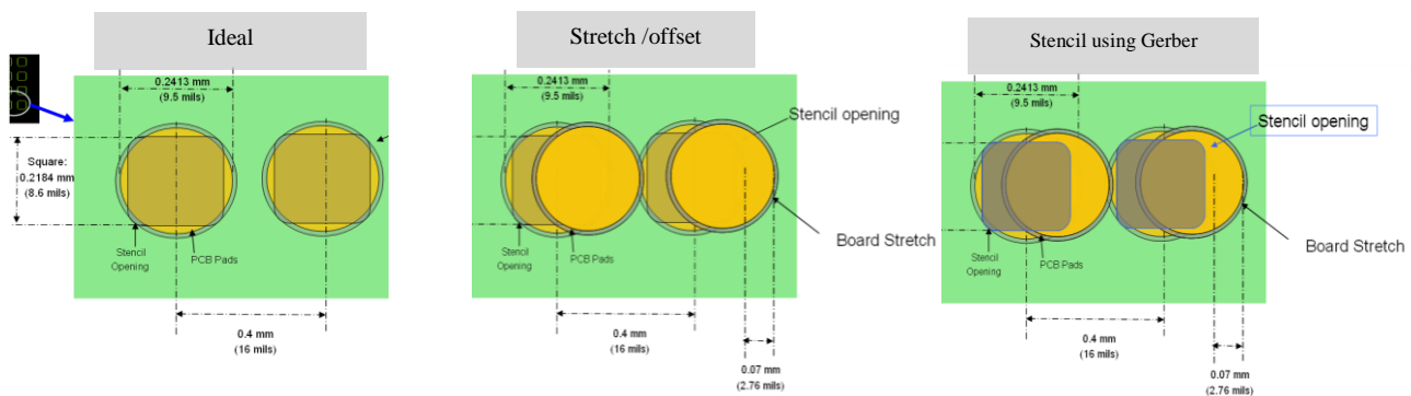
Figure 29: Stencils opening vs. PCB pad: represents the ideal world (CAD) and the consequences of the panel PCB stretch / offset.
