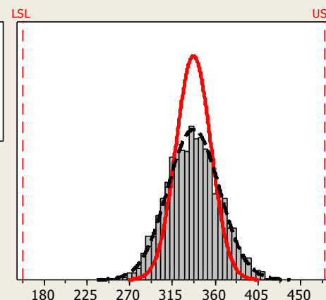
Process Capability of Nano coated CSP "A" Volume
