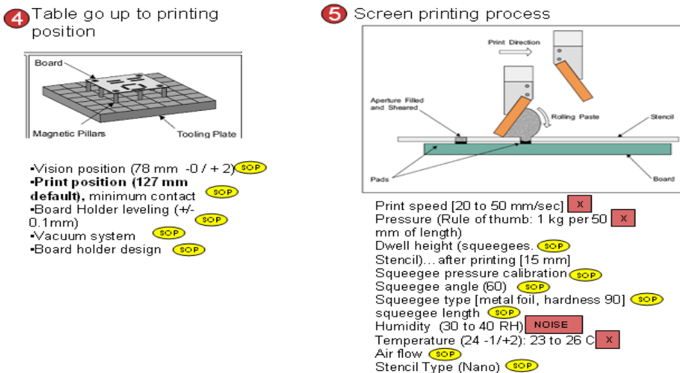
Figure2: 4 th & 5 th step of the printing process.
