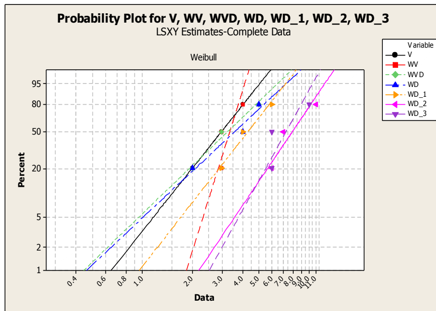
Figure 20: Weibull probability plot per type of cleaning settings: Y axis it's the defect % and X axis represent cleaning frequency. (Lot size: 83 panels).
