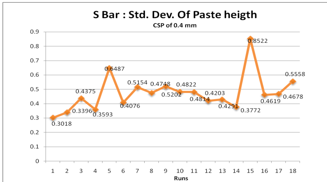
Figure 37: Standard deviation of the paste height by every DoE Run (in mils), sample size: 1152 boards (Lower values obtained are in the range of 0.3018 to 0.3772).
