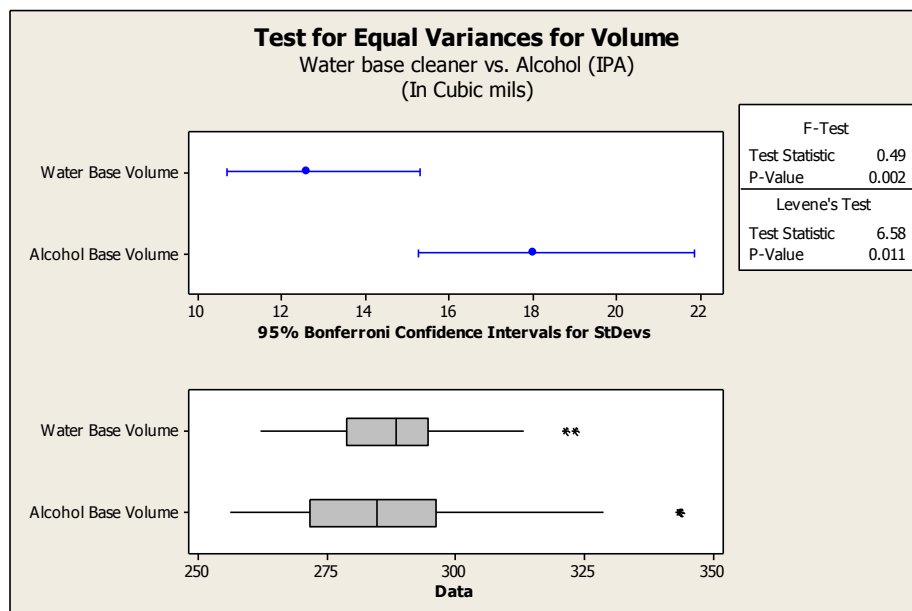
Figure 26: The test for equal Variance tells if the processes compared are similar or not: Water base cleaner demonstrate less dispersion of data (lot size: 557 panels = 2228 PCA’s).
