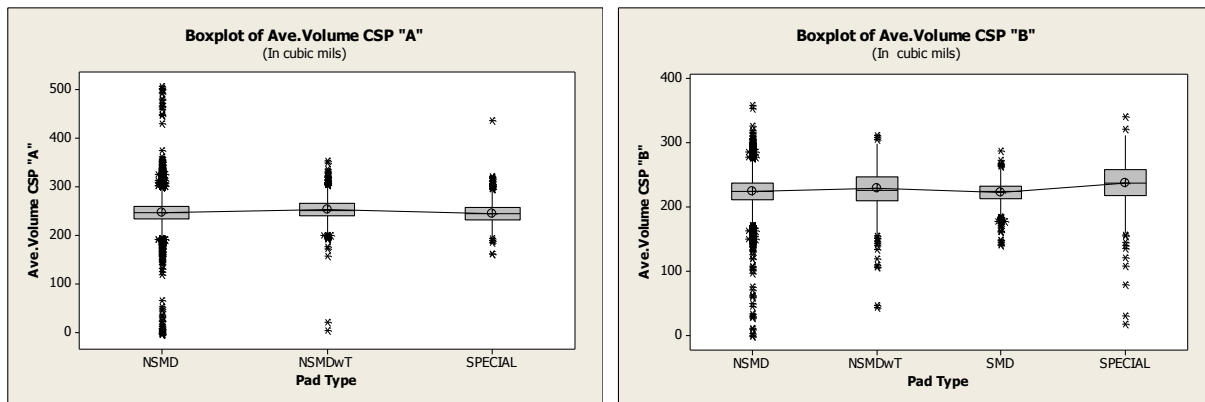
Figure 32: Paste volume deposit performance by pad type of CSP “A” & “B”. (Sample size: 298 panels)
