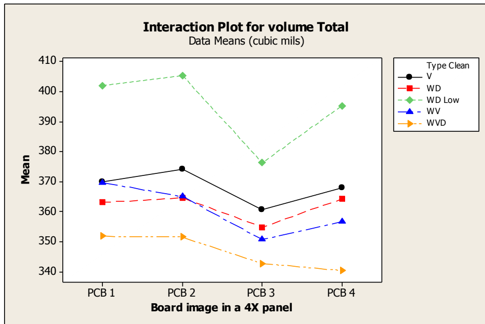
Figure 18: Print performance on “Volume” per images of the panel (Lot size: 83 panels).
