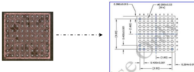
Figure 6: Bottom side of one of the CSP analyze with pitch on 0.4 mm, CSP solder ball of 0.26 +/-0.03 mm
