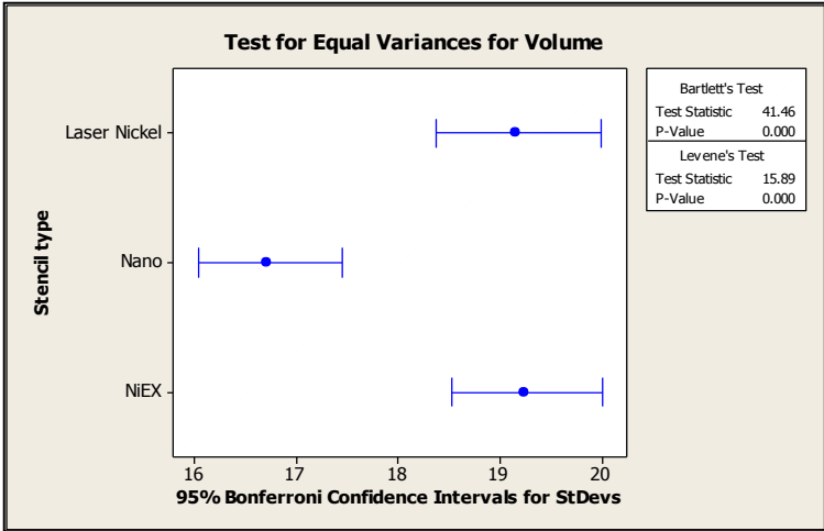
Figure 12: Stencil technologies Test for equal variance comparison. (Lot size: 720 units).
