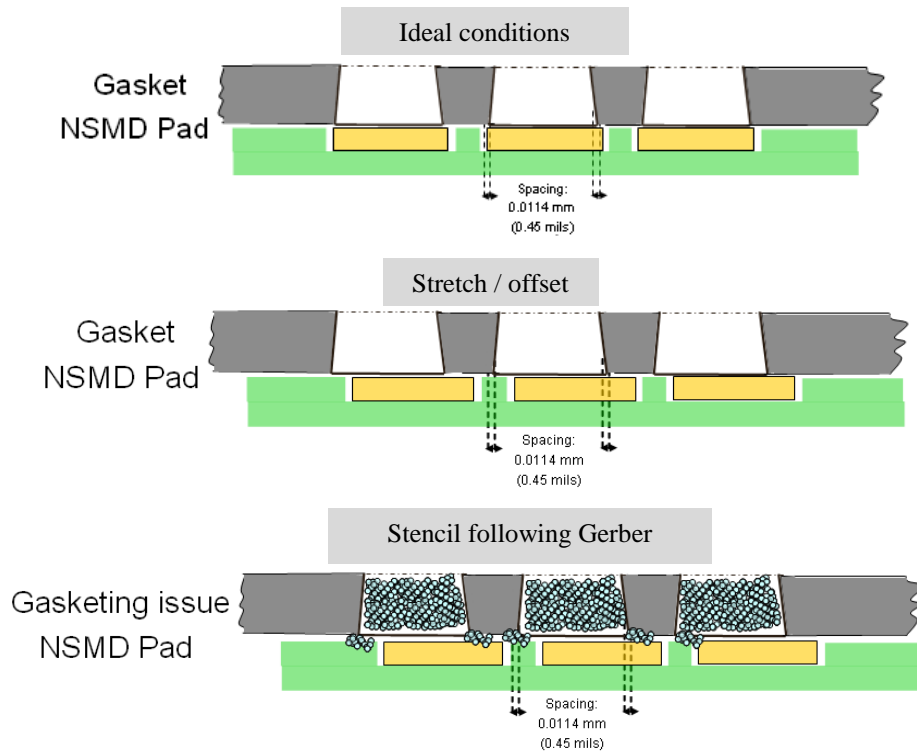
Figure 30: Gasketing issue between stencil & PCB pads.
