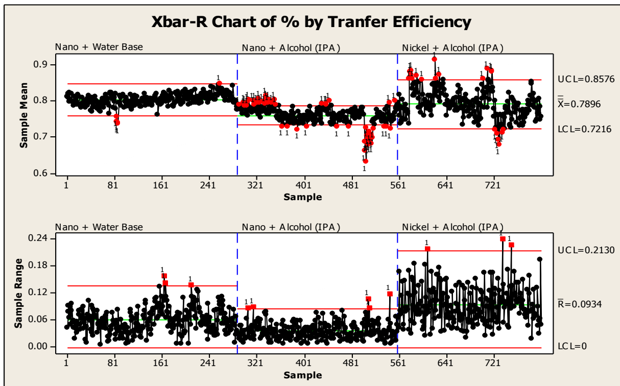
Figure 25: X bar charts used to compare “Transfer Efficiency” between Water & IPA using Nano (The Nickel laser cut use IPA as cleaner [lot size: 800 Panels, 3200 PCA’s]).
