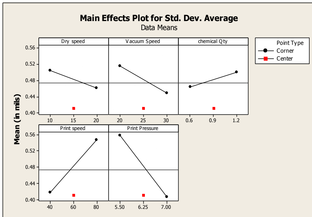
Figure 38: Main effect behavior of the DoE: Printing variables Vs Cleaning Variables.
