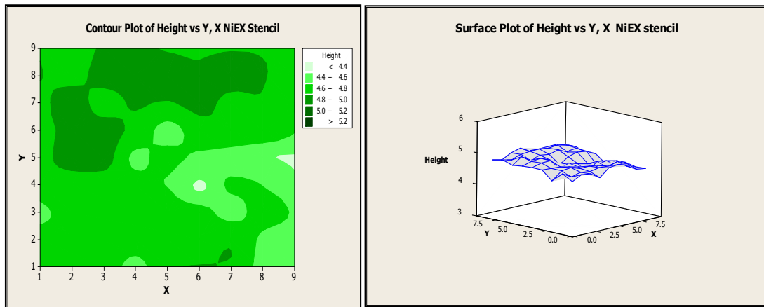
Figure 15: E Fab (NiEX): Paste height distributions along the 0.4 mm pitch CSP (in mils). Lot size: 240 PCA.
