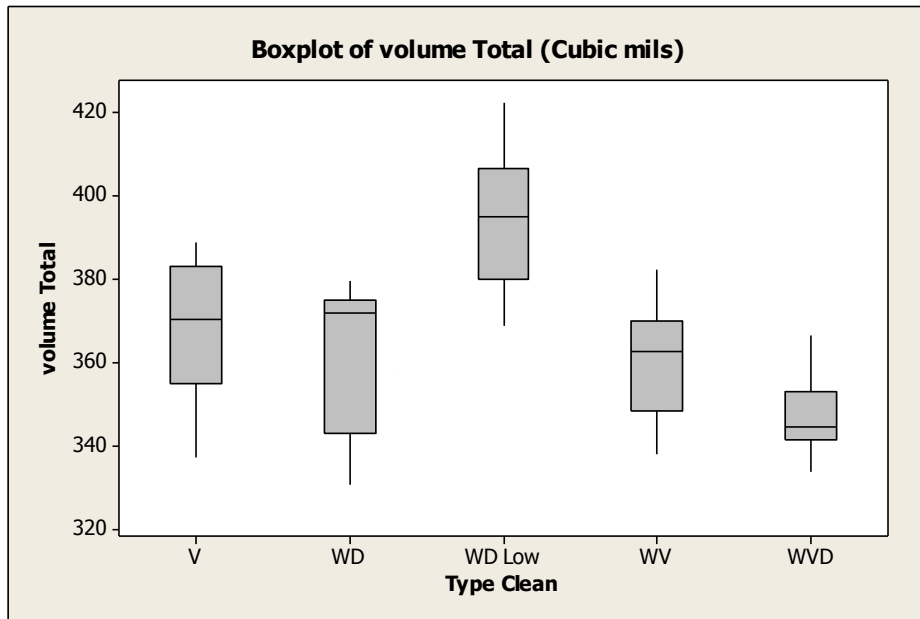
Figure 17: Volume box plot performance per type of cleaning settings (Lot size: 83 panels).
