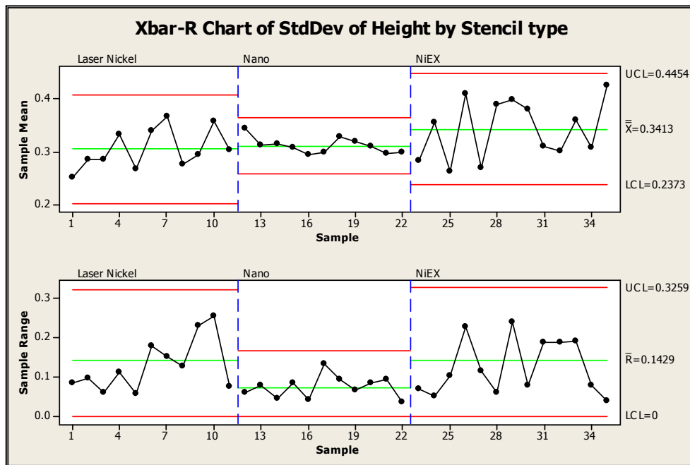
Figure10: Xbar R chart for Std. Dev. of height in mils (lot size: 720 units per stencil type).
