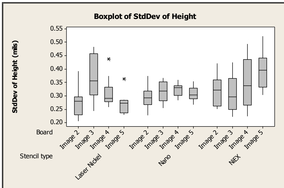
Figure11: Box of paste height per PCA image and Stencil technology (lot size: 720 PCA's, 240 per stencil type).
