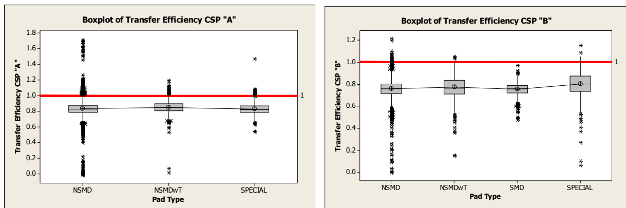
Figure 33: TE Performance by pad type for both CSP’s of pitch of 0.4 mm. (Sample size: 298 panels)
