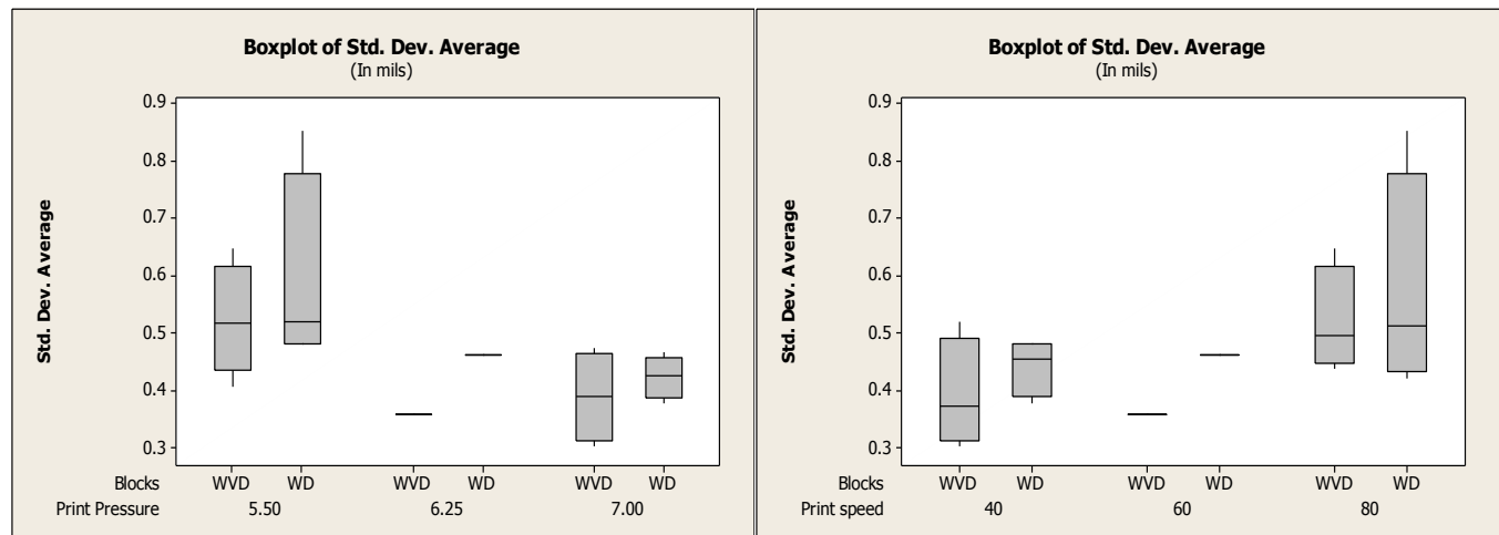
Figure 41: DoE Block behavior: WVD vs. WD: Print pressure & Print speed (sample size: 1152 boards).
