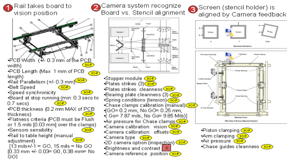
Figure 1: 1 st 2 nd & 3 rd step of the printing process.
