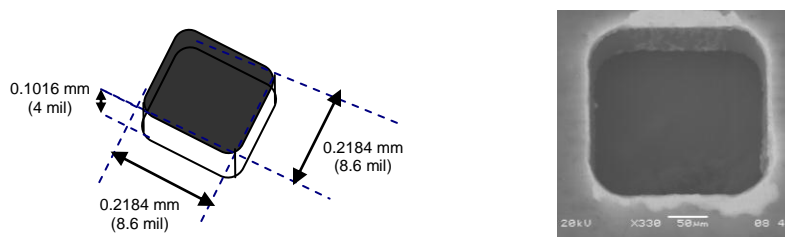
Figure 24: Stencil opening analyzed with the Nano coated stencil.
