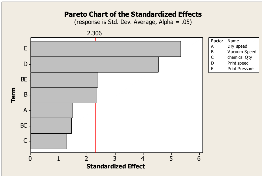
Figure 39: More important factor that affects the printing performance & process repeatability.
