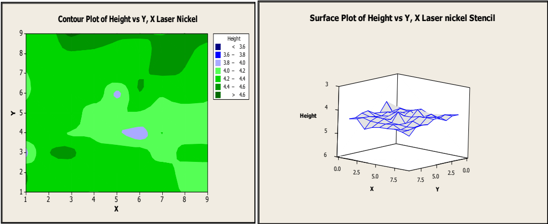
Figure 13: Laser Nickel stencil: paste height distribution along the 0.4 mm pitch CSP (in mils). Lot size: 240 PCA
