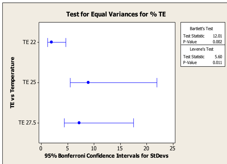
Figure 45: Transfer efficiency test for equal variance for all stencil openings. (Sample size: 192 panels)
