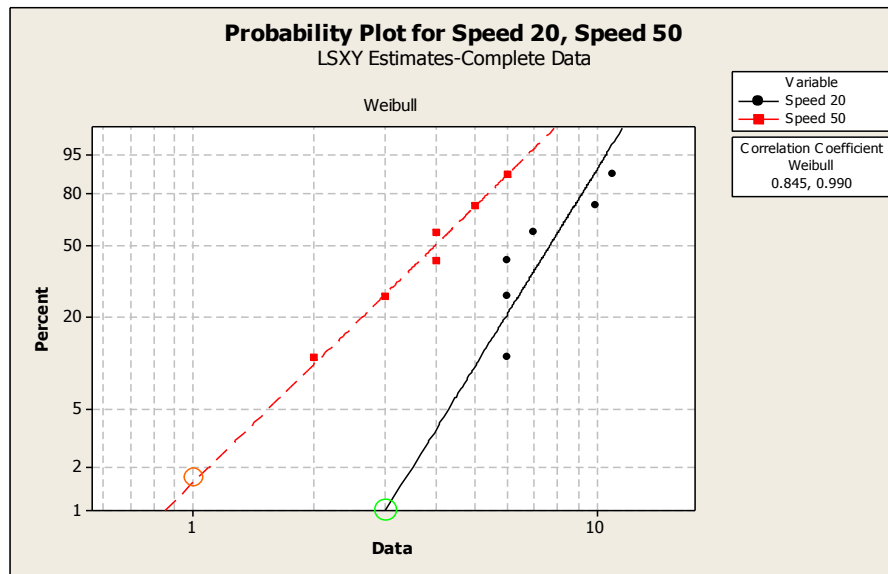
Figure 21: Weibull plot prediction for 2 cleaning speeds of 20 & 50 mm/sec using a WD setting (Wet-Dry cleaning). (Lot size: 83 panels).
