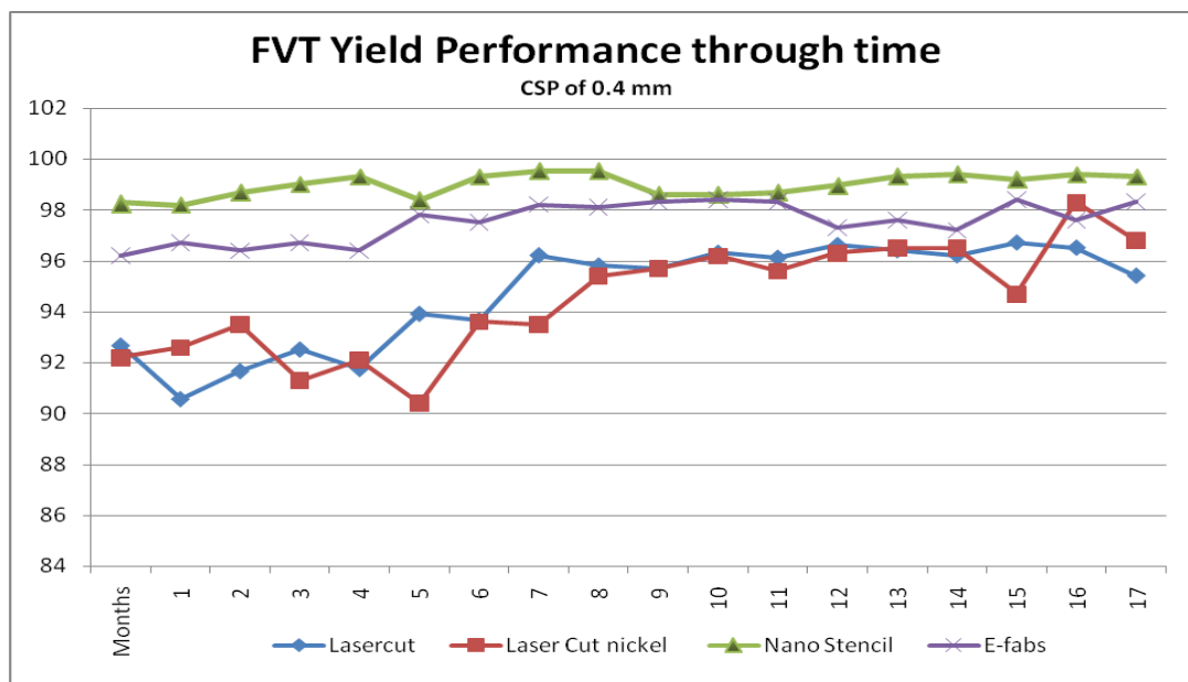
Figure 16: General yield trend on FVT per type of stencil (CSP of 0.4 mm pitch).
