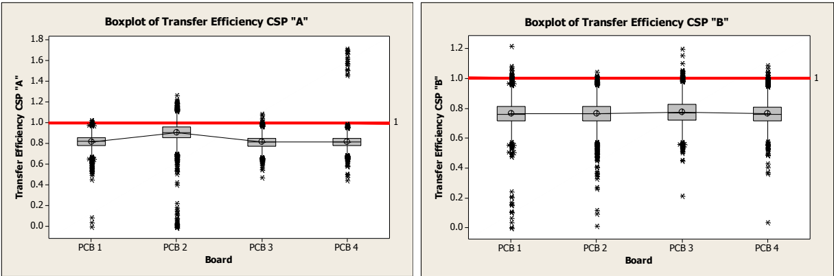
Figure 34: TE Performance by image of the panel of 4X, the CSP “A” with 88% of NSMD becomes the most sensitive. (Sample size: 298 panels)
