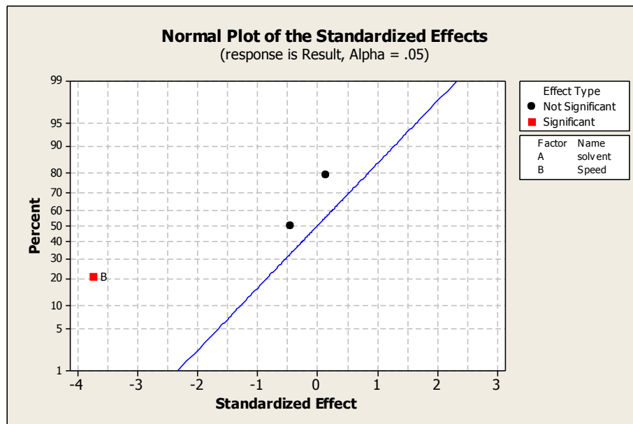
Figure 22: Significant effects: Cleaner & Speed: Speed (red square) its more distance form the blue line, while the black spots (A) represent the solvent used is not significant. (Lot size: 83 panels).
