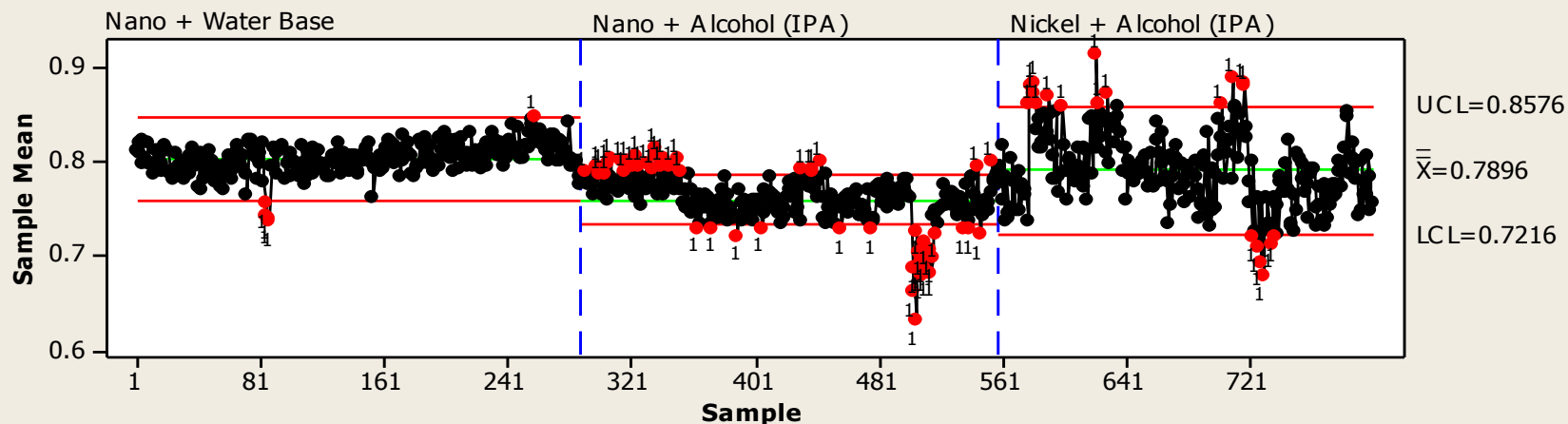
Xbar-R Chart of % by Transfer Efficiency
