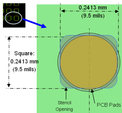
Figure 7: Close up of stencil opening design for Nickel laser cut.
