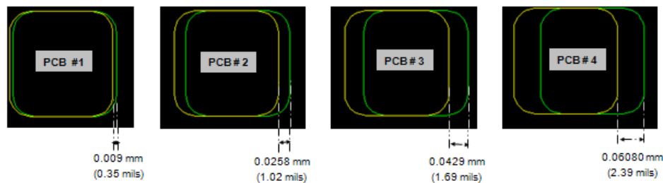
Figure 27: Measurements made on panels of 4X where the stretch increase along the panel. Stretching occurs mostly on the “X” axis rather than the “Y” axis.
