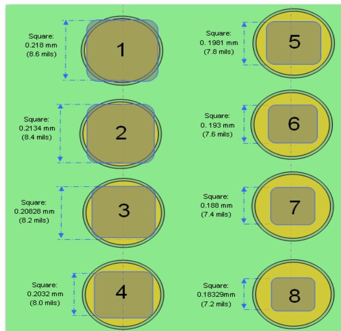
Figure 43: Different stencil designs analyzed (one per each board, on a stencil with double image).
