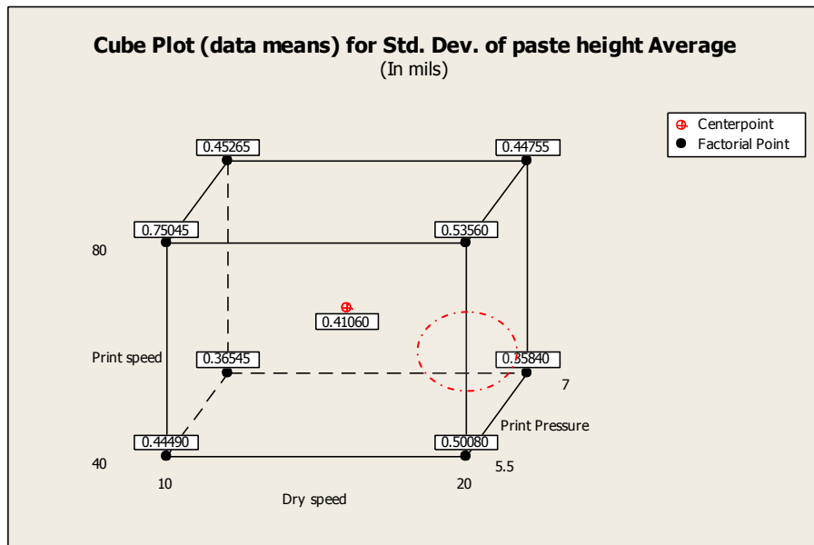
Figure 40 illustrates the variables interaction in a cube plot, the lowest standard deviation is 0.3540. (Sample size: 1152 boards).
