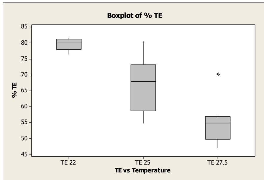
Figure 44: Transfer efficiency performance vs. temperature using all the stencil openings (sample size: 192 panels)
