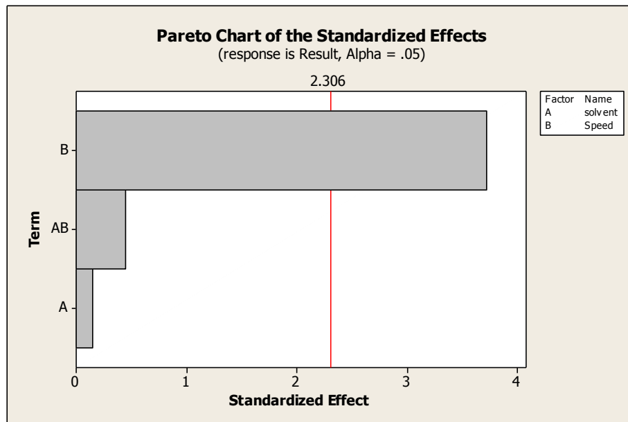
Figure 23: Main effects: Speed becomes more important in this stage of the experiment. (Lot size: 83 panels).
