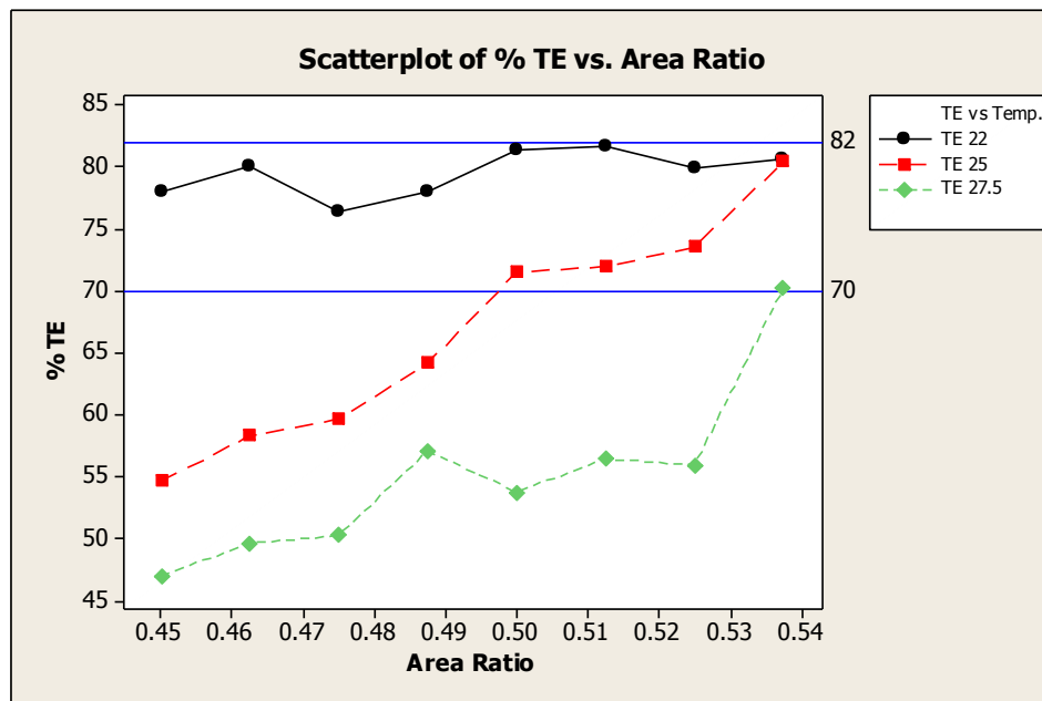
Figure 46: TE vs. Area ratio performance by Temperature (sample size: 192 panels).
