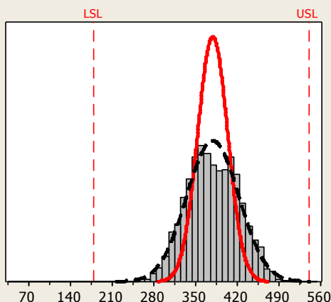
Process Capability of laser cut CSP "A" Volume
