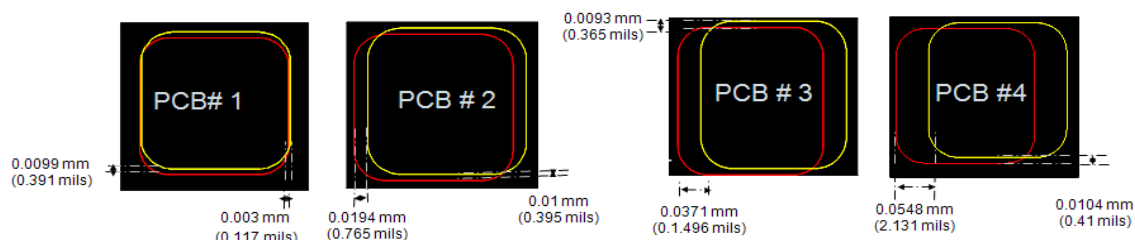
Figure 28: Measurements of the PCB stretch /Offset on a 4X panel
