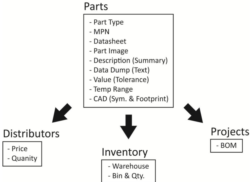
Figure 8 – A simplified view of the FriedParts data storage schema. Part parameters are reduced to a generic minimum. Further type-specific parameters are stored in a searchable text block rather than as explicit database fields to simplify the data entry automation.
