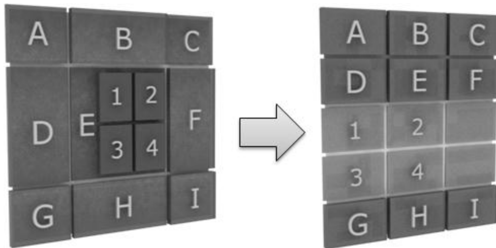
Figure 11 - A diagrammatic view of FriedParts' table refactoring.
