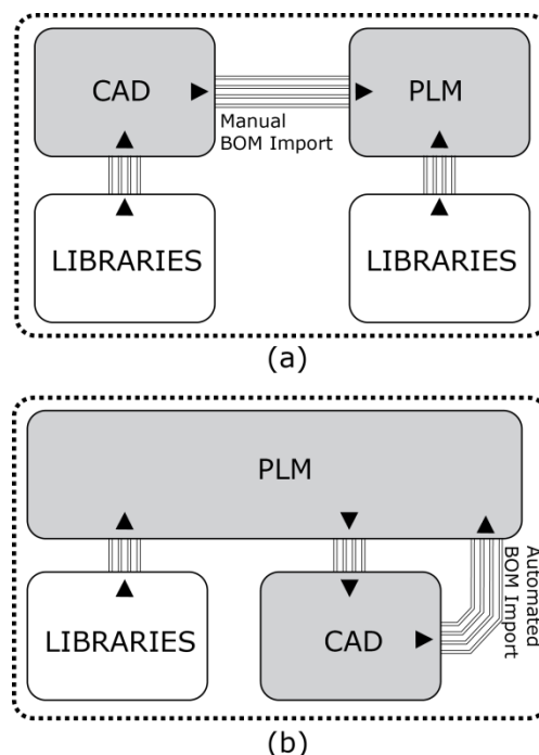
Figure 5 – (a) Current CAD tool to PLM tool interaction. Note the manual BOM alignment step during import/update to the PLM tool. (b) Proposed tool interaction approach – FriedParts. By eliminating the CAD tool's direct control of its libraries and bringing all user interaction to the PLM, CAD-to-PLM BOM interactions are automated since the CAD tool is already using PLM-aware parts.
