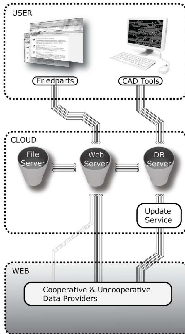
Figure 6 – The FriedParts’ system architecture. The core infrastructure is divided into four cloud-hosted components which combine to run the website and manage its data.
