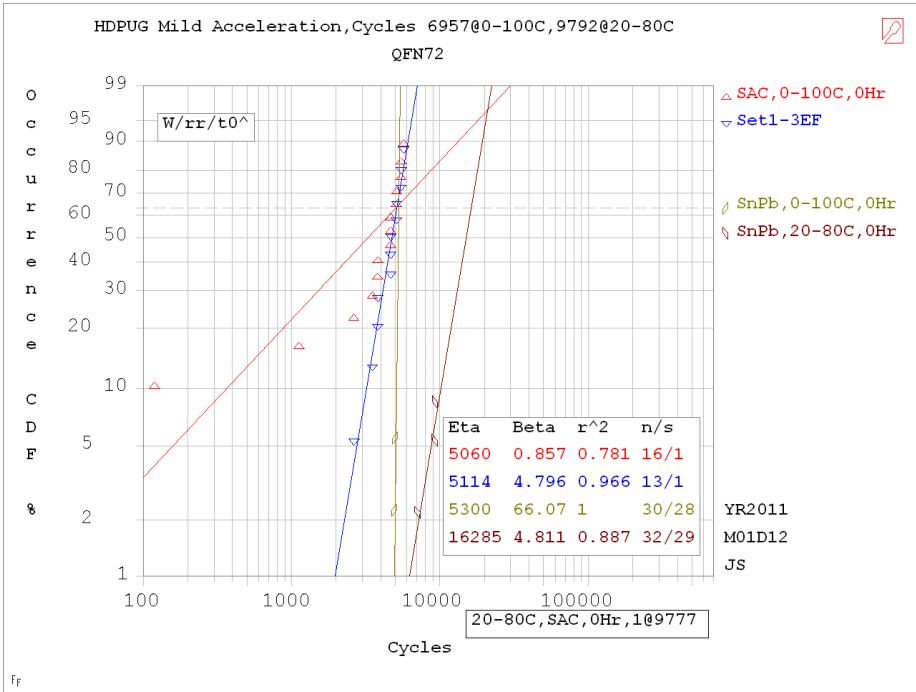
Figure 18: Weibull plots of the QFN 72 thermal cycle failure data
