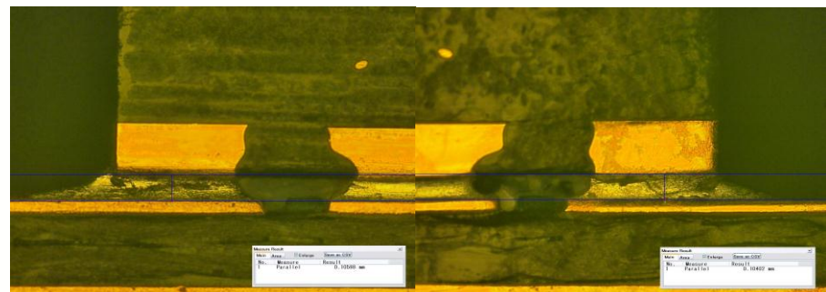
QFN64, Assembled with SAC solder, failed at 84 cycles in 0-100° C thermal cycling
