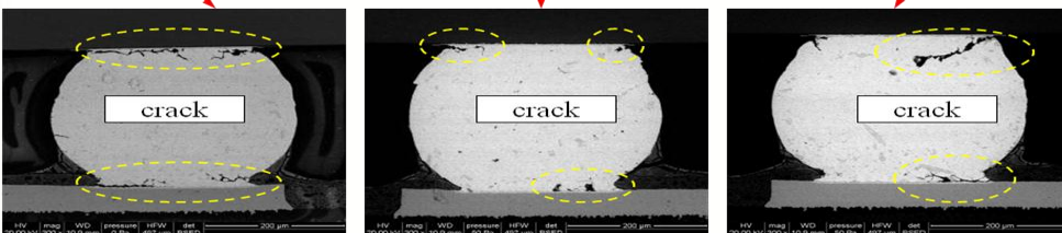
WSBGA 54, assembled with SAC solder, failed at 1639 cycles in 0-100° C thermal cycling
