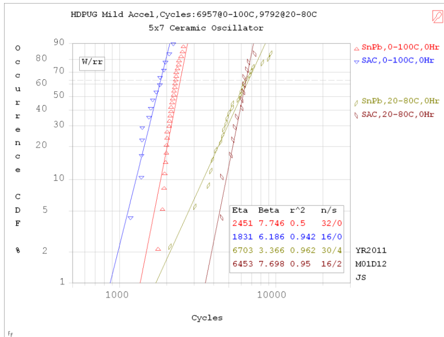
Figure 8: Weibull plots of the 5 x 7 mm ceramic oscillator thermal cycle failures
