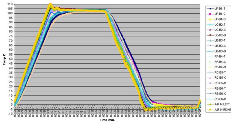
Figure 5: Thermal profile for the standard 0-100°C accelerated temperature cycle
