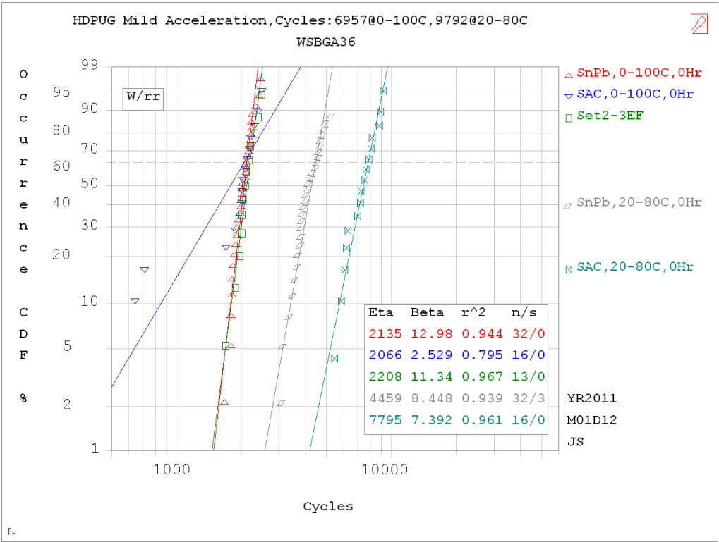
Figure 20: Weibull plots of the WSBGA 36 thermal cycle failure data
