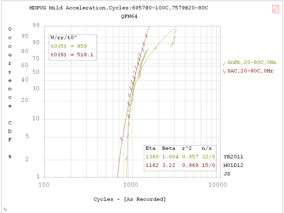
Figure 17: 3 Parameter Weibull plots of the QFN 64 failure data in 20-80°C thermal cycling
