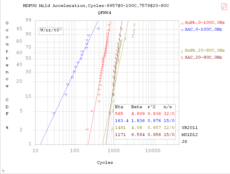
Figure 16: Weibull plots of the QFN 64 thermal cycle failure data
