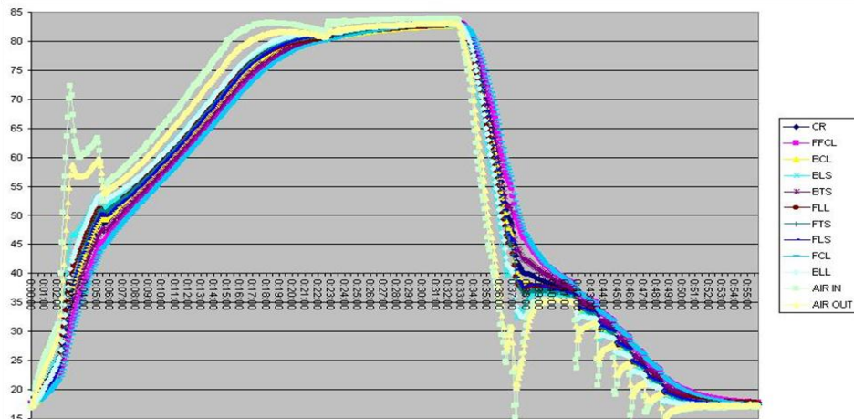
0-100° C Thermal Cycle
