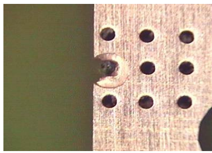
Missing copper
