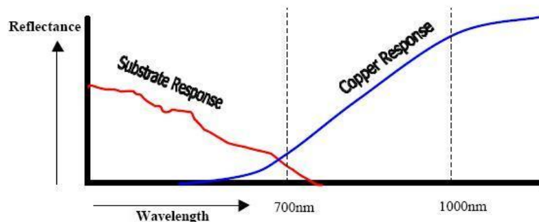
Figure 14 – Reflectance vs Wavelength
