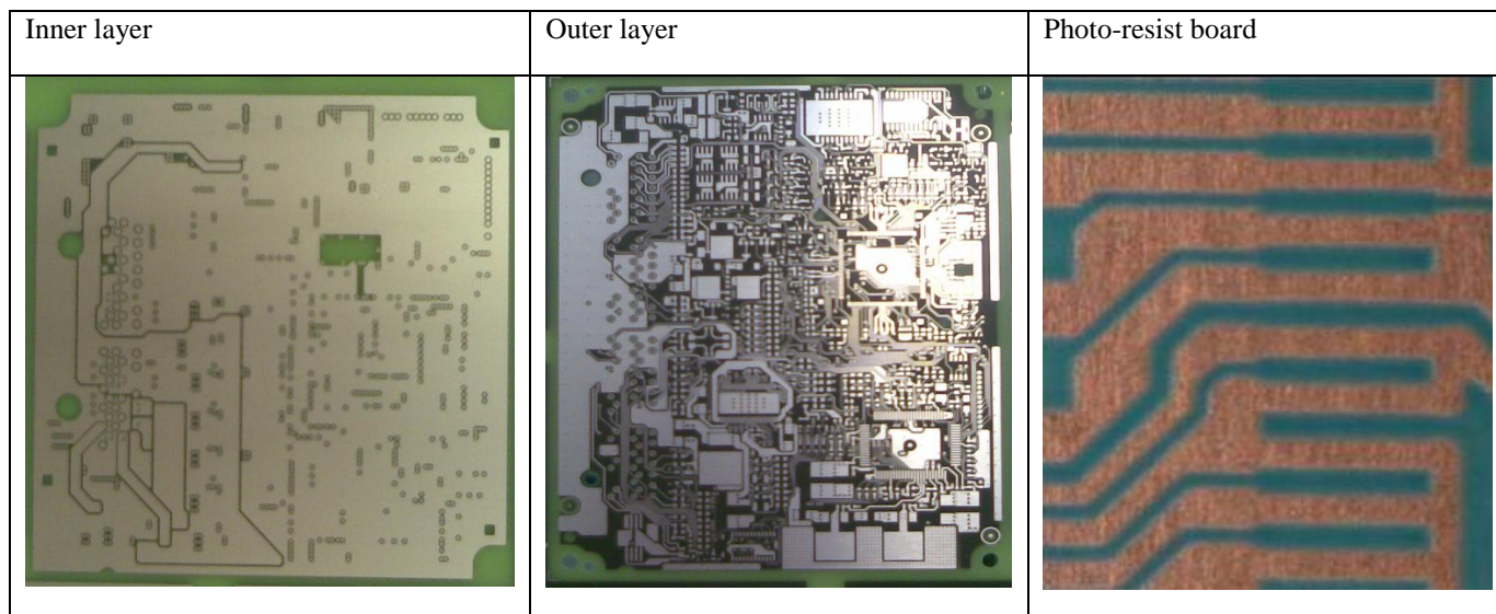
Figure 5 – AOI target boards
