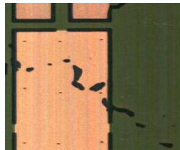
Solder mask Ink on pad
