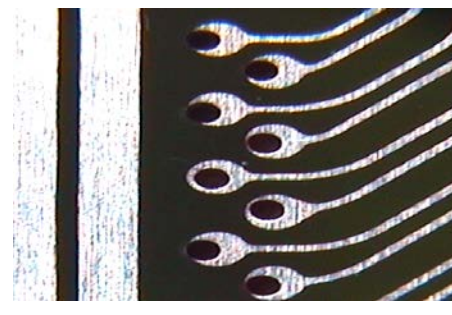
Hole misalignment
