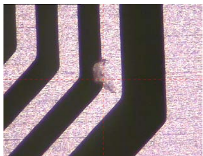
Excess copper
