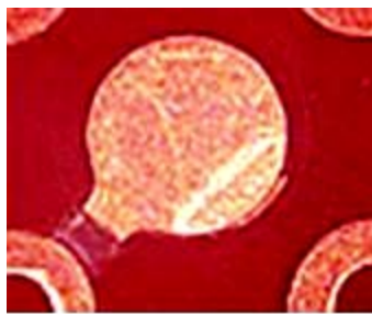
Dent on pad
