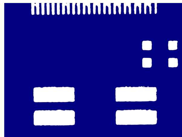
segmentation results
