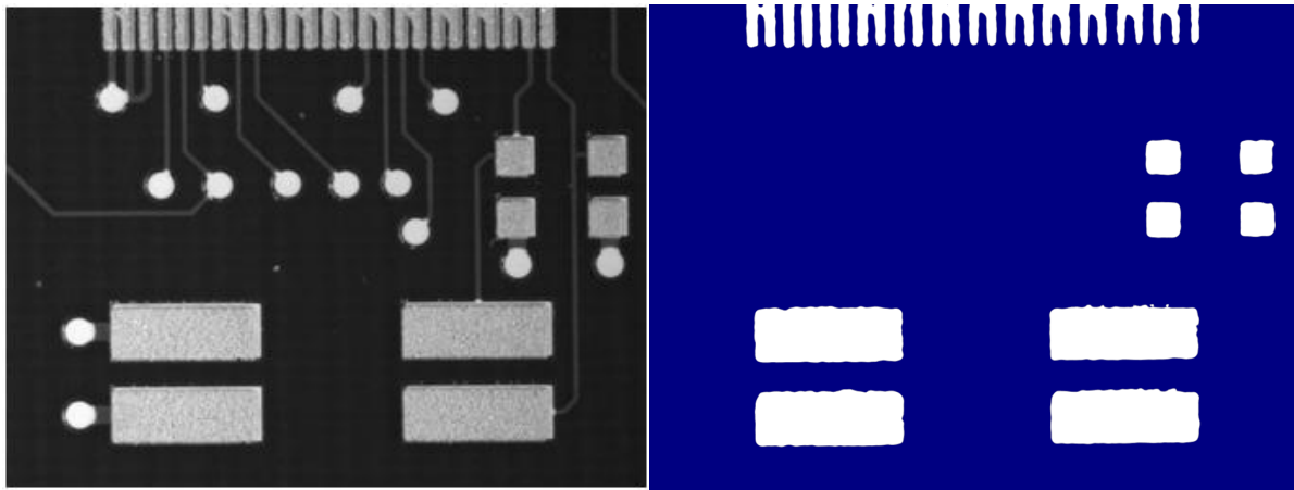
Figure 9 – Solder paste image and segmentation results
