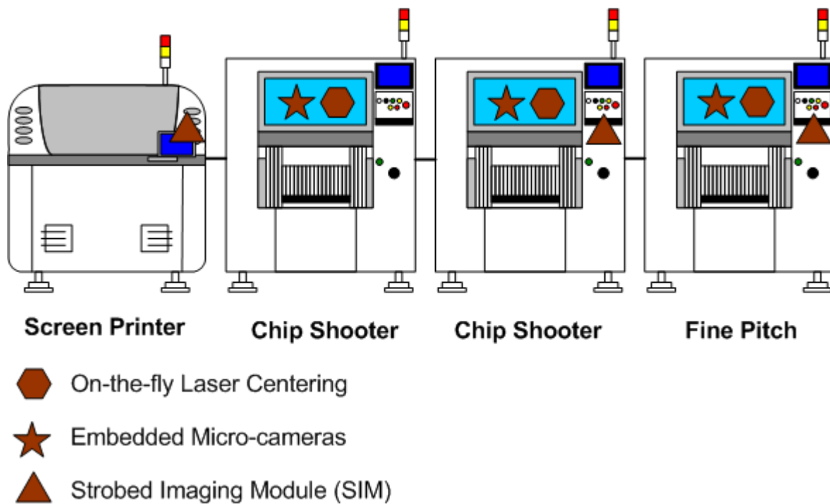
Figure 1 – SMT assembly line showing embedded sensor locations
