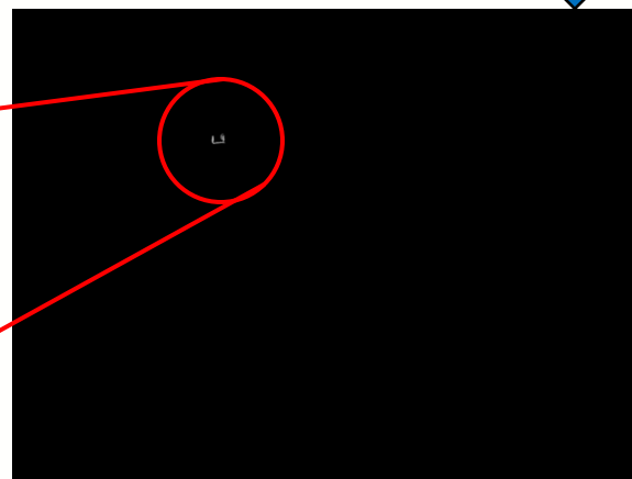
difference image
