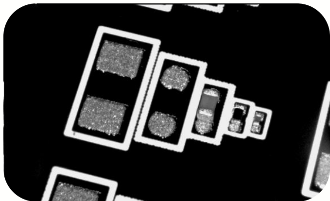
before image
