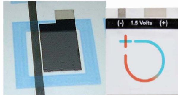
Blue Spark Technologies: Printed Battery
