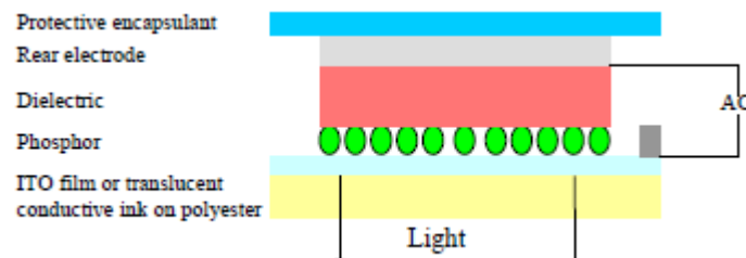
Figure 3 – Electroluminescent Lamp
