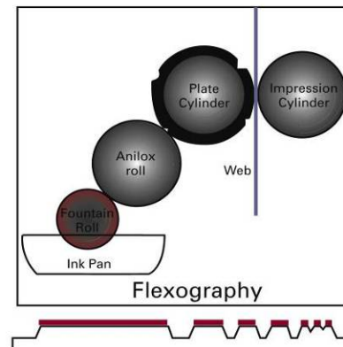
Flexography - Relief
