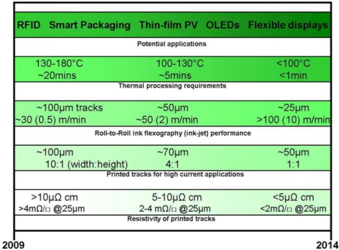
Figure 7. An outline of some future development paths for printed conductive materials
