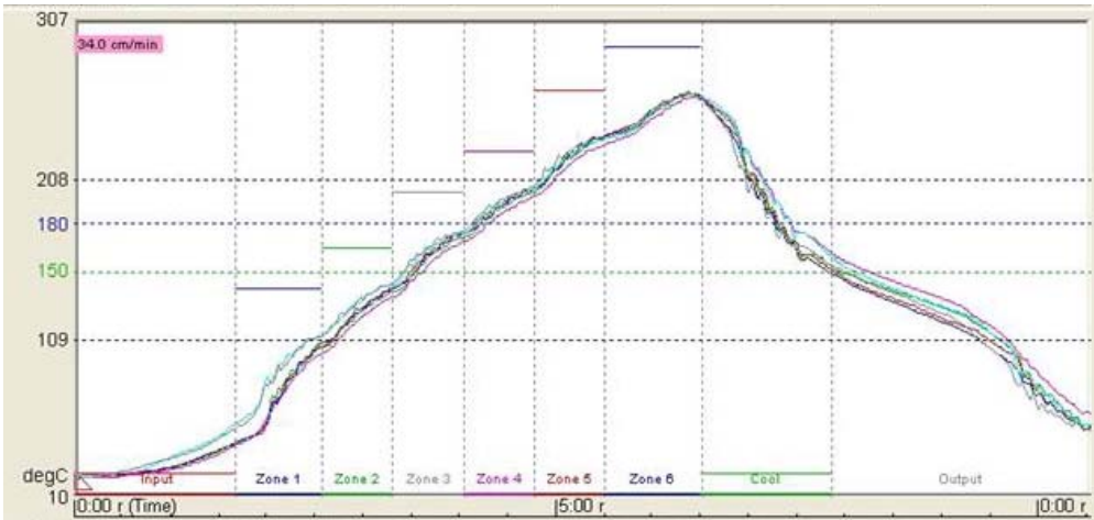
Figure 3. Typical lead-free soldering reflow cycle.
