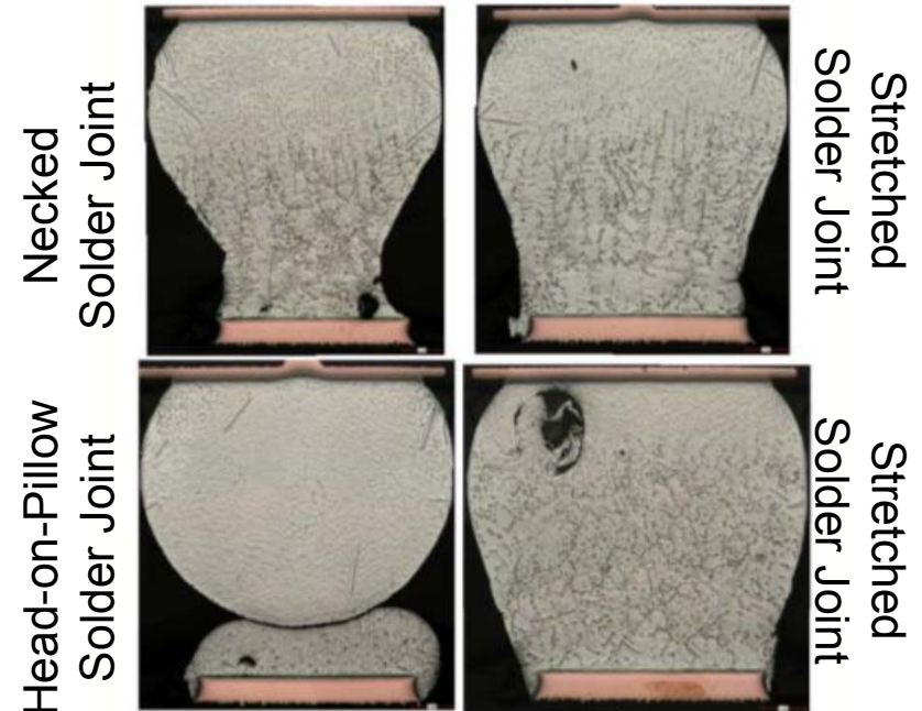
Optical Micrographs for Leg 1 Early Failures
