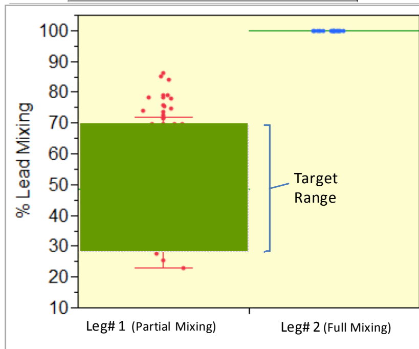
Box Plots for Leg 1 and Leg 2
