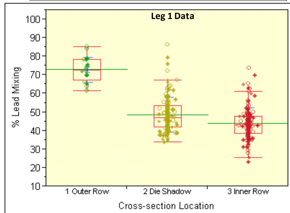
Box Plots for Leg 1 for each row measured
