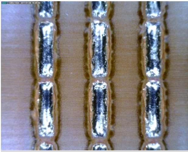
Figure 3a. Wetting pattern for testing for SAC387
