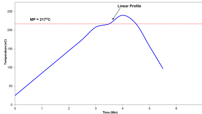
SAC Alloy Reflow Profile
