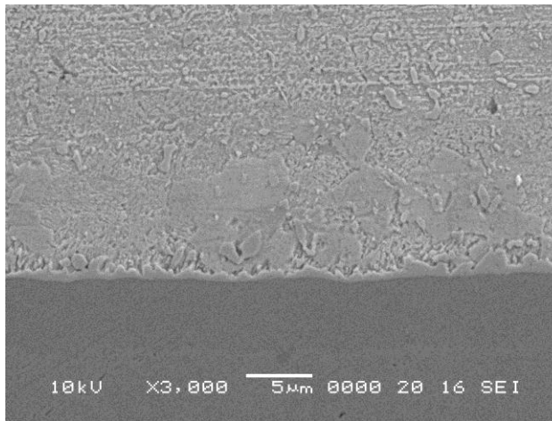
Figure 6b. An etched SAC105 solder joint
