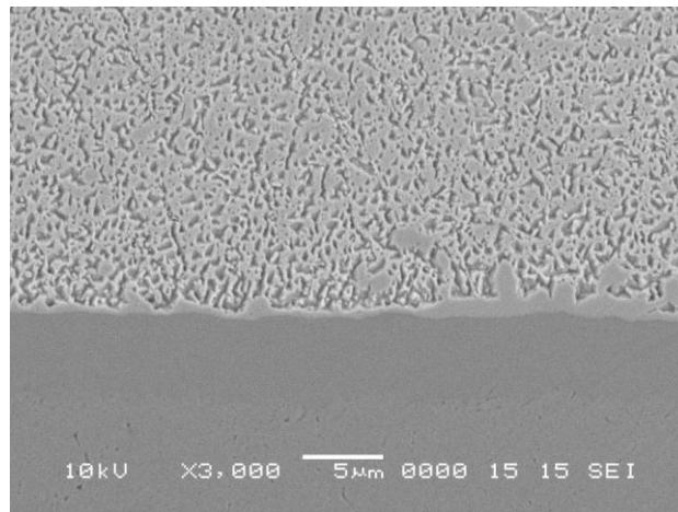
Figure 6a. An etched SAC305 solder joint.
