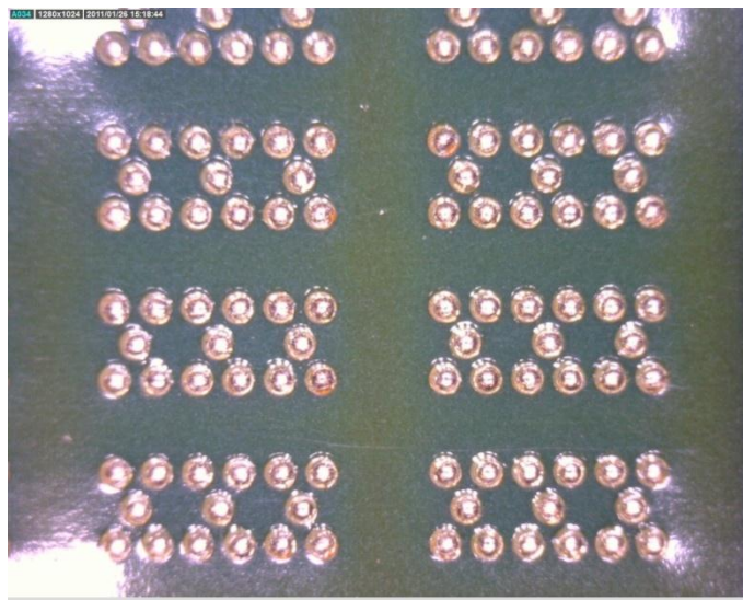
Figure 4b. Small deposits visually inspected for coalescence for SAC387
