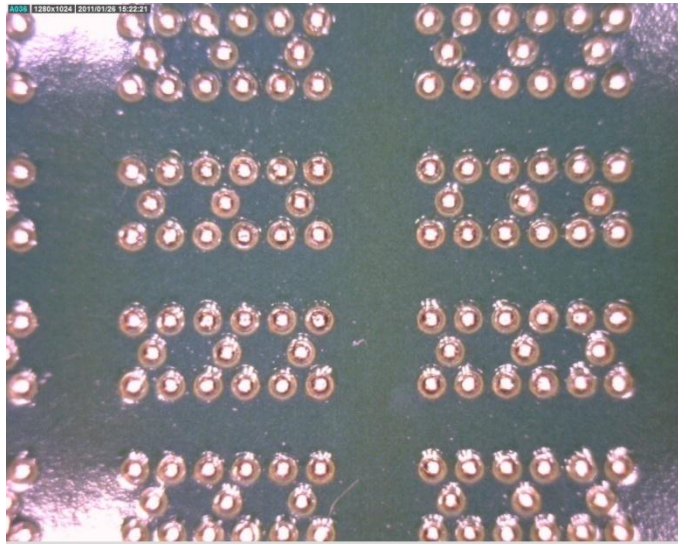
Figure 4b. Small deposits visually inspected for coalescence for Sn992
