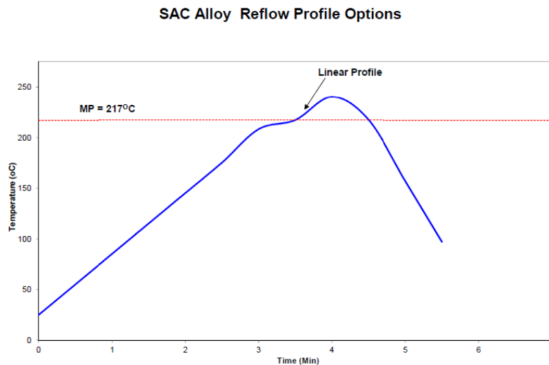
Figure 5. Typical SAC305 linear reflow profile
