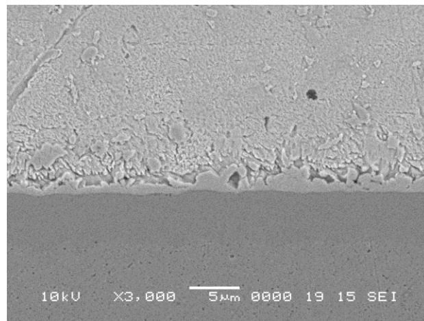
Figure 6c. An etched SAC0307 solder joint.
