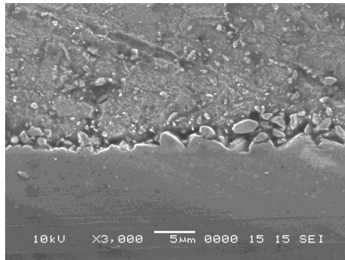
Figure 6d. An etched Sn992 solder joint.
