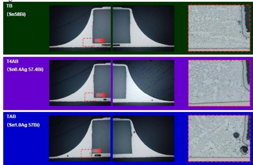
Figure 26: Sn58Bi, Sn57.6Bi0.4Ag and Sn57Bi1Ag soldered 3216 [1206] chip component cross-sections.
