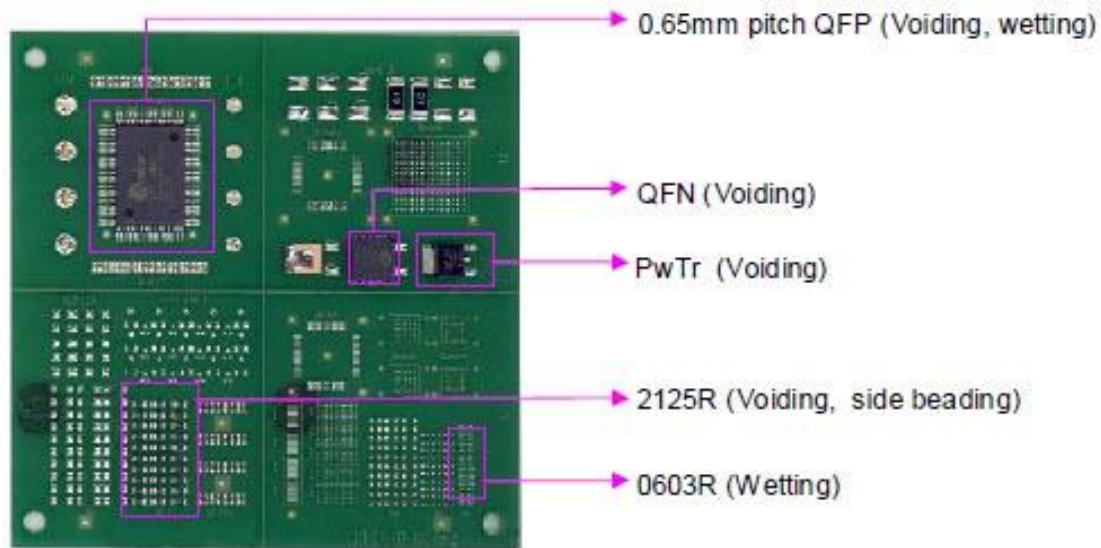
Figure 2: Solder reflow test vehicle.
