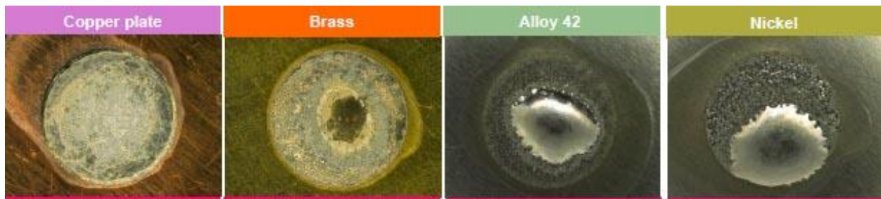
Figure 12: Sn58Bi Type paste A reflow spreading on Copper, Brass, Alloy 42 and Nickel material test pieces.
