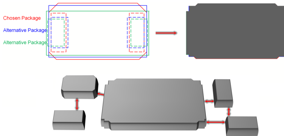
Figure 2 – Enveloping takes into account the “worst case” size of all possible components.
