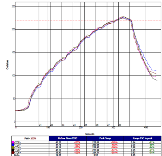
Standard Profile for Test Vehicle II
