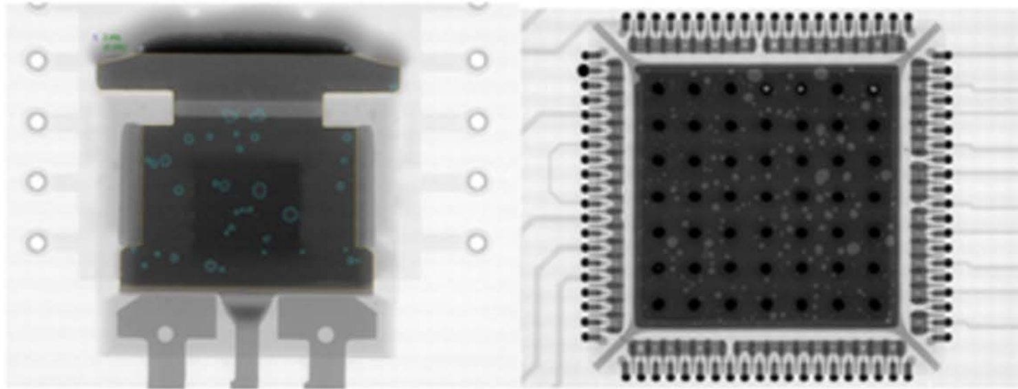
D-PAK with weight
