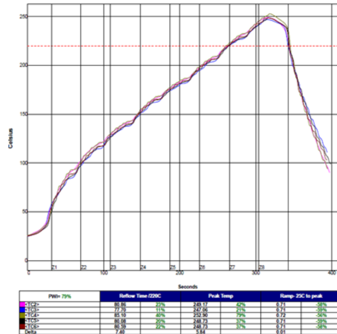
Hot Profile for Test Vehicle II
