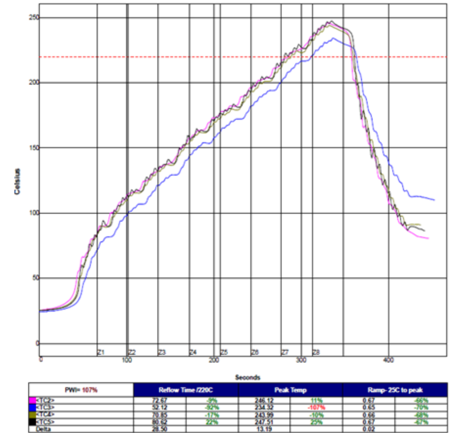
Hot Profile for Test Vehicle I with Cu Weights
