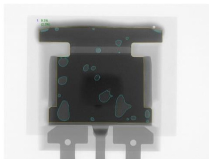
Figure 13 Component A, ENIG, no variable
