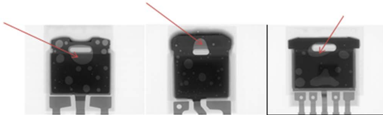
Voiding occurring around mold filled openings in thermal pad
