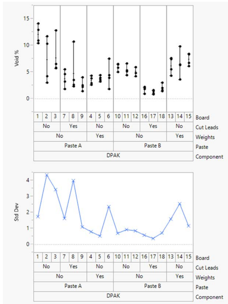
D-PAKs Only, No QFNs
