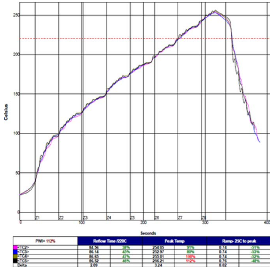
Hot Profile for Test Vehicle I
