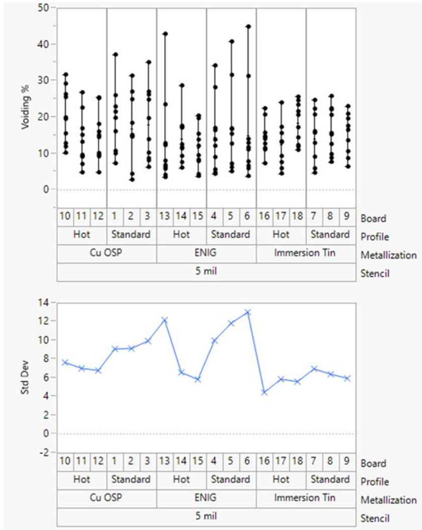
Boards 1-18 comparing reflow profile
