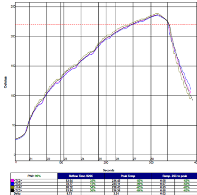
Standard Profile for Test Vehicle II
