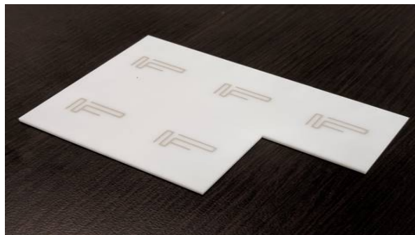
Figure 9 – Jetted lines of conductive paste; approximately 300µm wide
