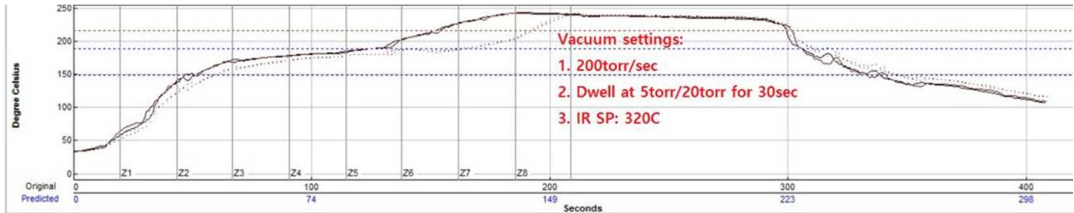
Profile Cooling Slope
