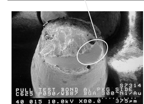
Ni/Au, Ball Failure Feature
