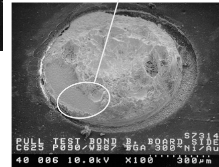
Ni/Au, Board Failure Feature
