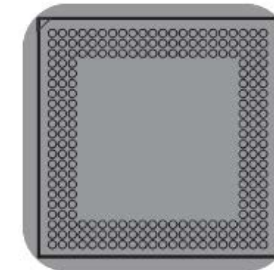
(a) Full underfill
