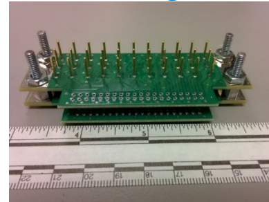
Specimen potting (12mm)
