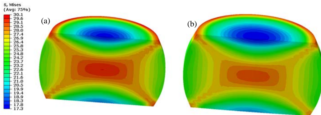
Figure 16 Von Mises stress plot in (a) center (b) corner joint for specimen with PM2 potting at the end of high temperature dwell of the 1 st cycle
