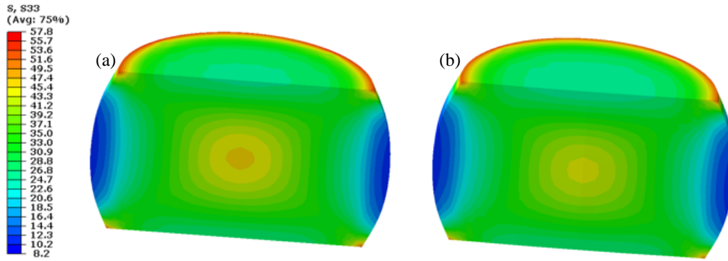
Figure 17 Axial stress plot in (a) center (b) corner joint for specimen with PM2 potting at the end of high temperature dwell of the 1 st cycle
