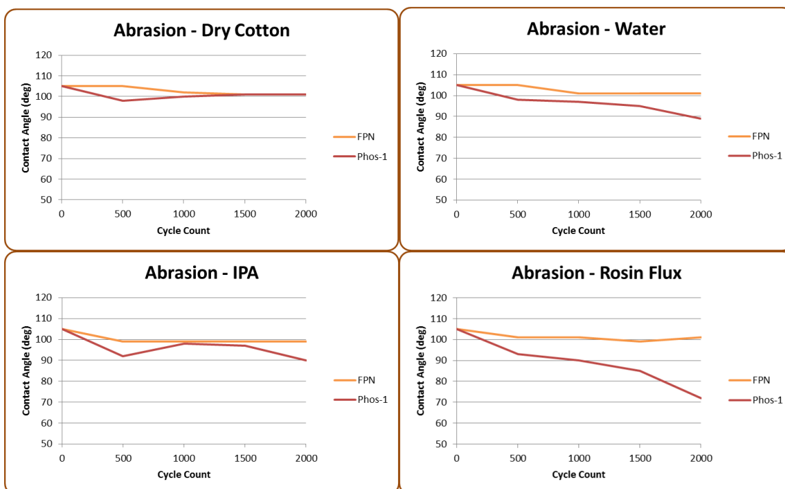
Figure 8: Contact Angle Over 2000 Scrub Cycles with Dry Cotton, DI Water, IPA, and Rosin Flux
