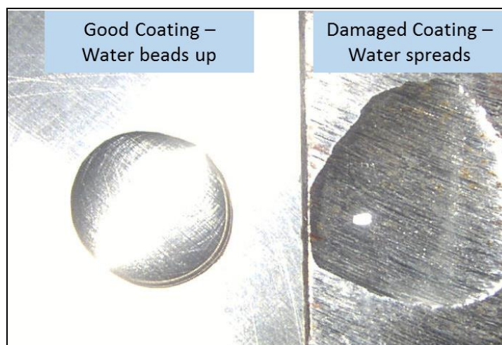
Figure 10: Fresh Coating (Good Hydrophobicity) and a Damaged Coating (Poor Hydrophobicity)
