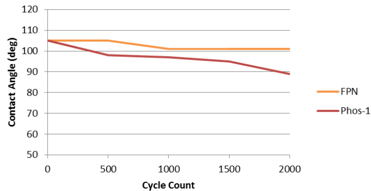
Abrasion - Water
