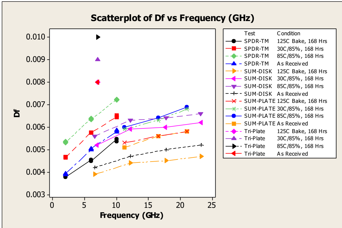
Figure 7: Df versus Frequency versus Moisture Content
