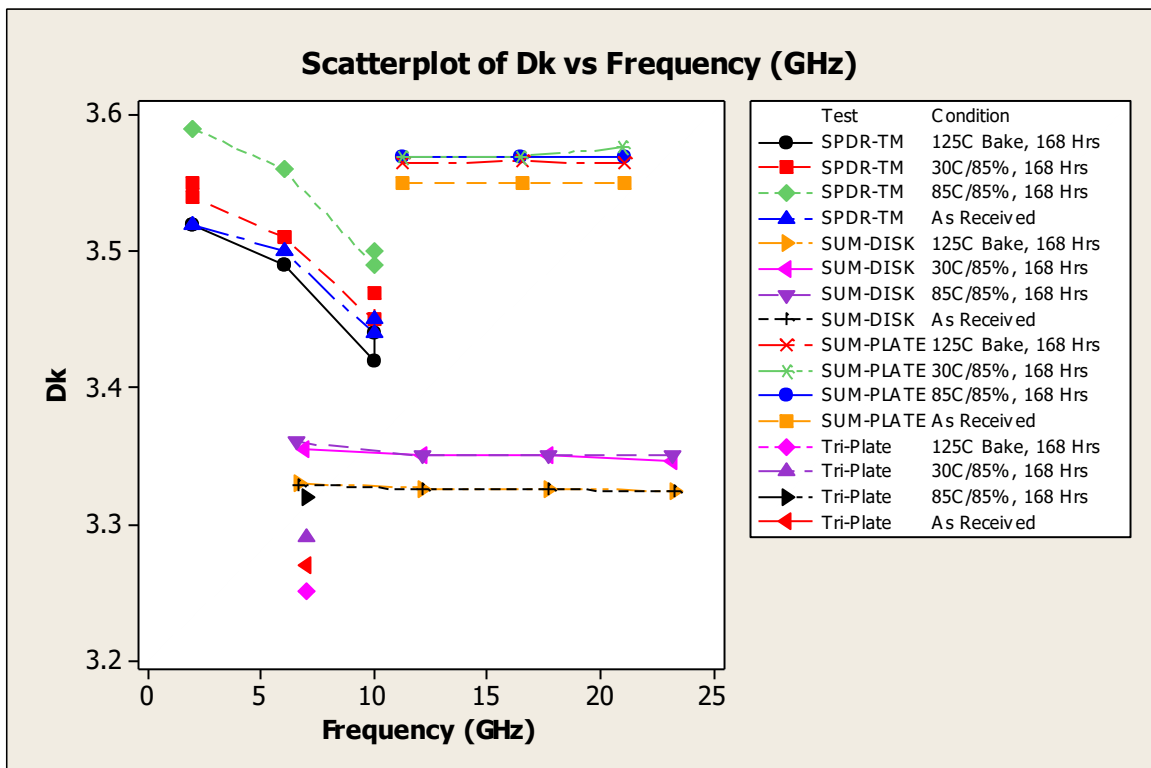
Figure 6: Dk versus Frequency versus Moisture Content
