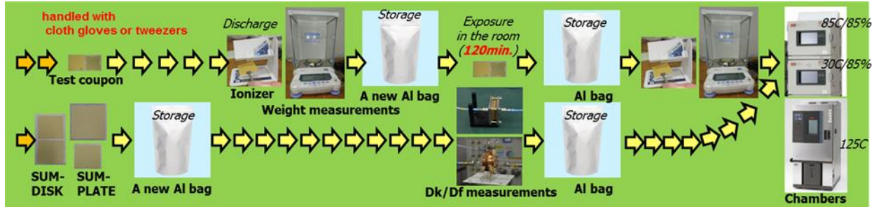
Figure 2: Process Flow for Weight Gain/Loss and Dk/Df Measurements
