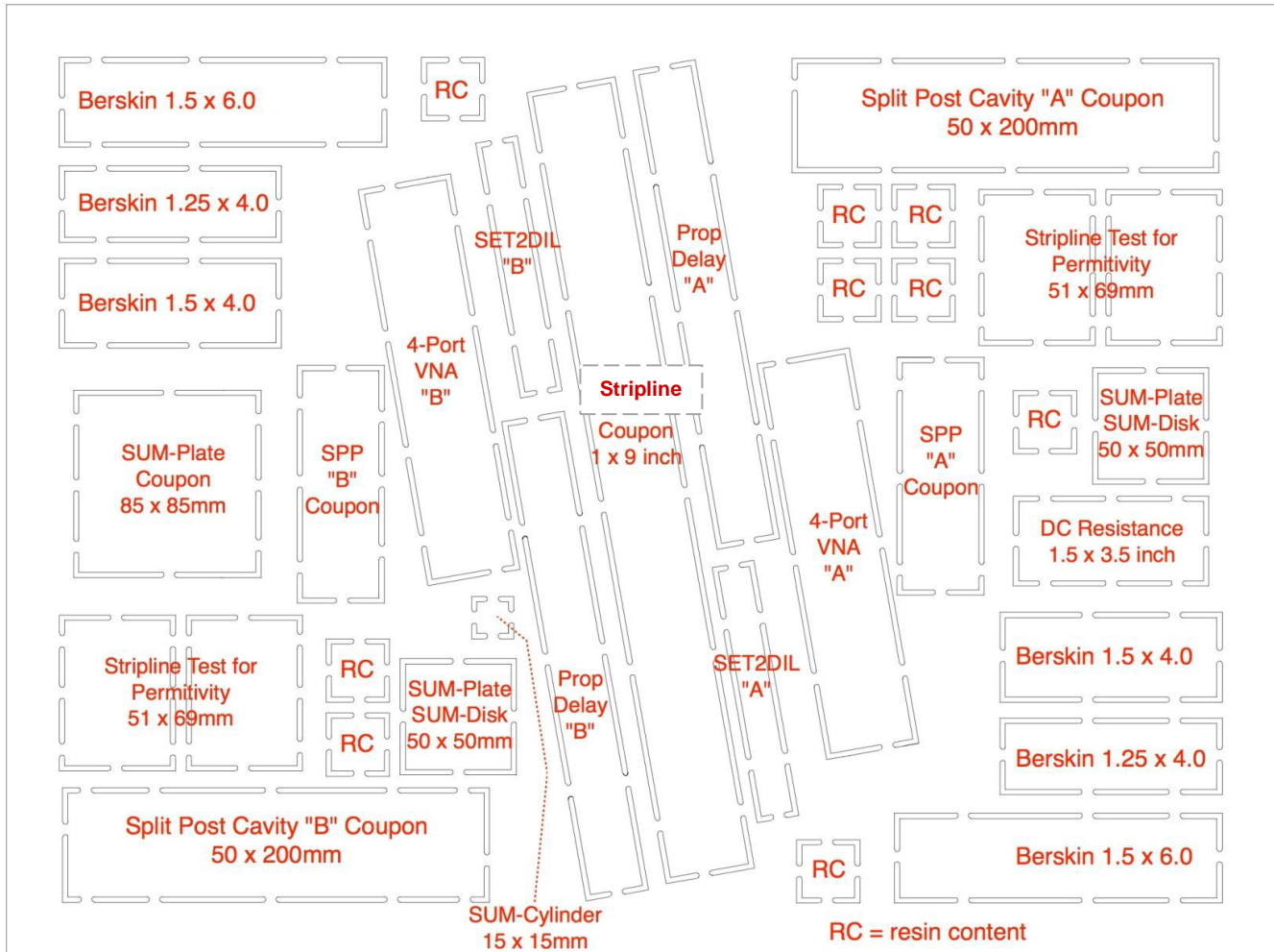
Figure 1: Phase 2 Test Board Layout
