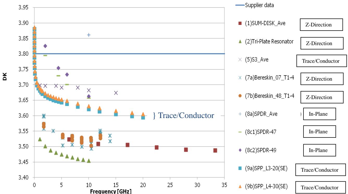
Figure 3 – Comparison of Dk Results by Test Method (for single material)
