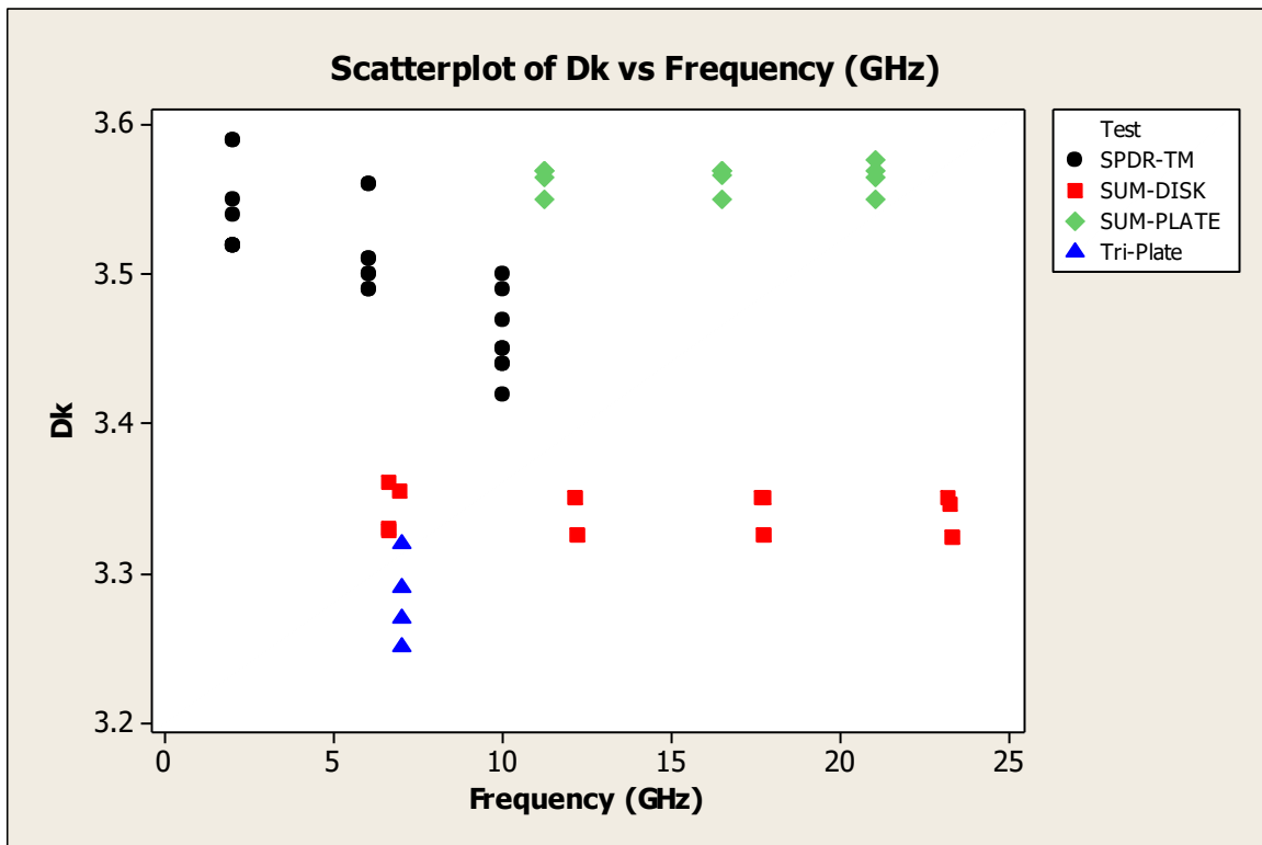
Figure 5: Dk versus Frequency
