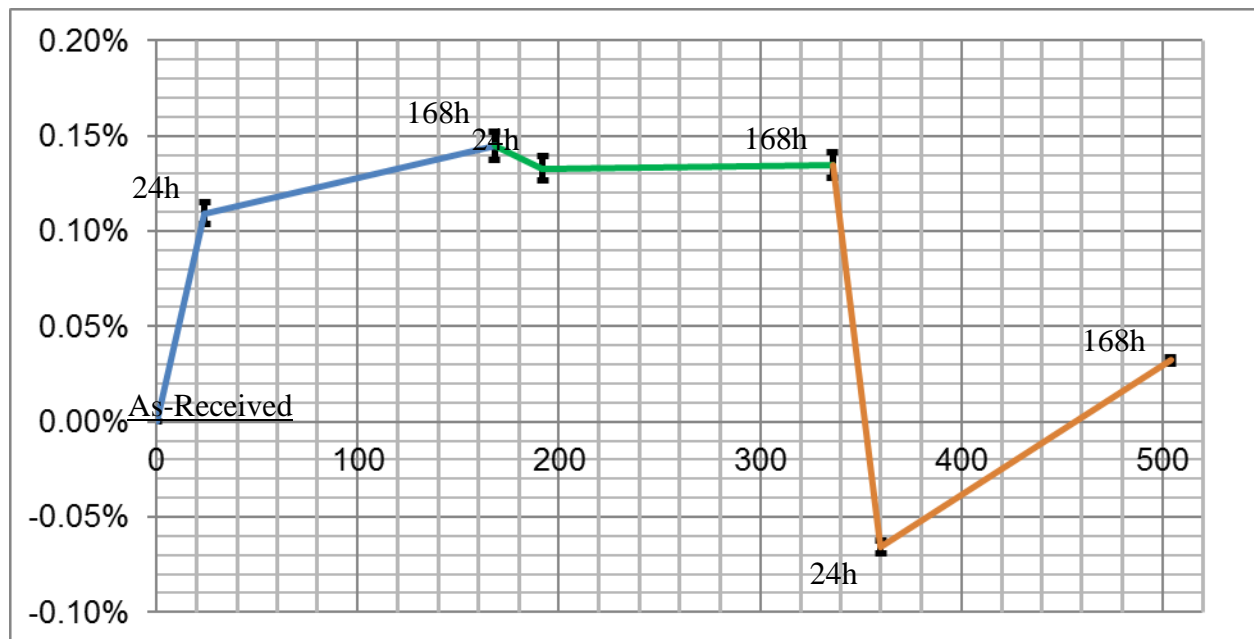
Figure 4: Relative Weight Change = (measured – as received) / (as received)
