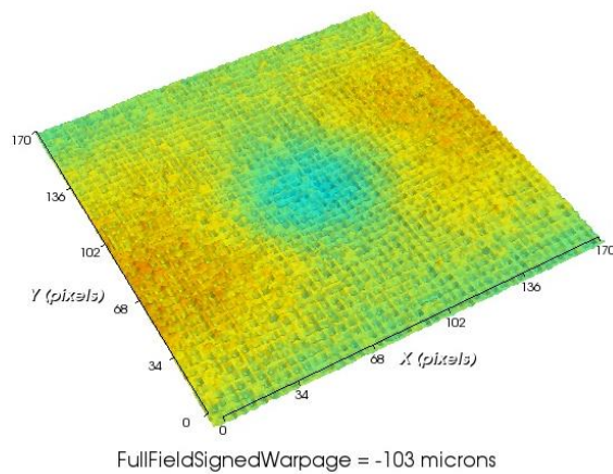
Figure 6a. Negative Saddle [5]
