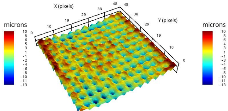
JFFS Warpage = -23 microns
