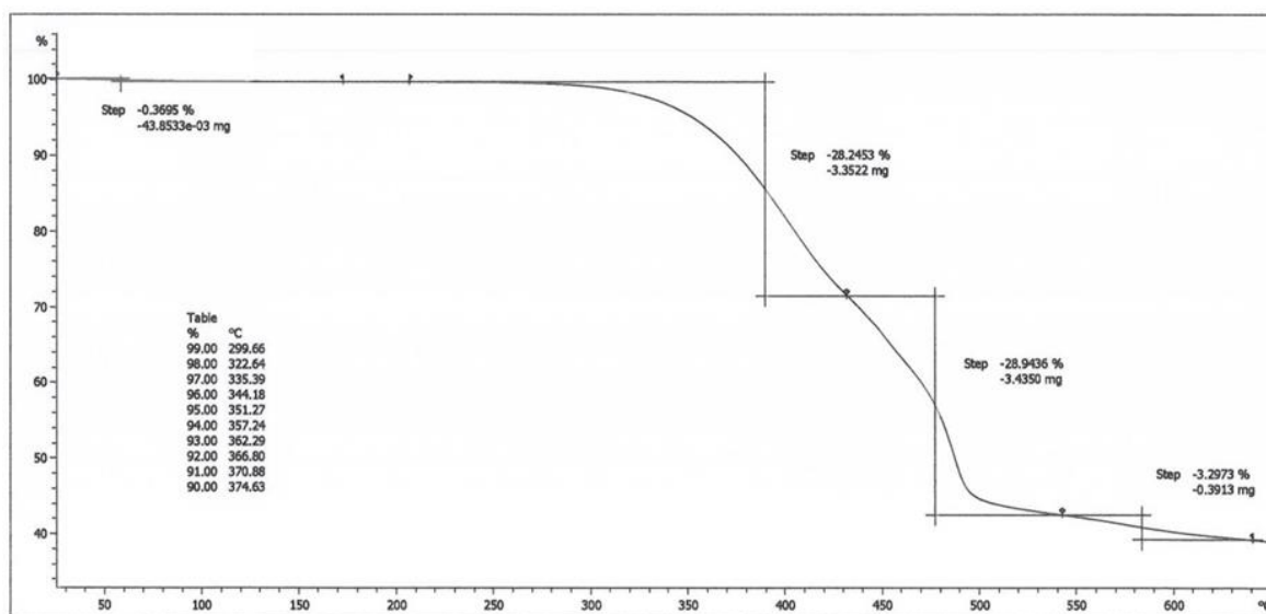
Figure 1 - TGA of Material A, Heating rate 10 C/min, nitrogen flow
