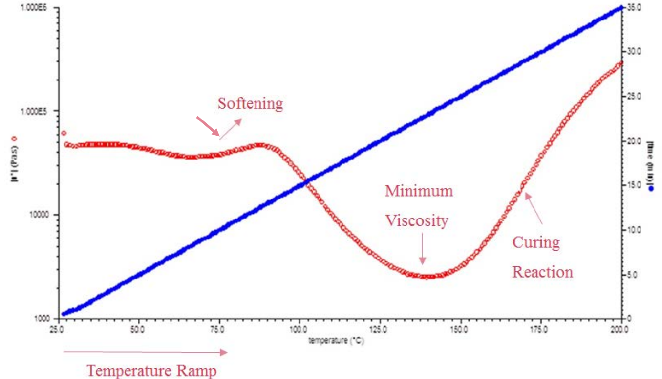
Complex viscosity profile of the prepreg at 5°C/min
