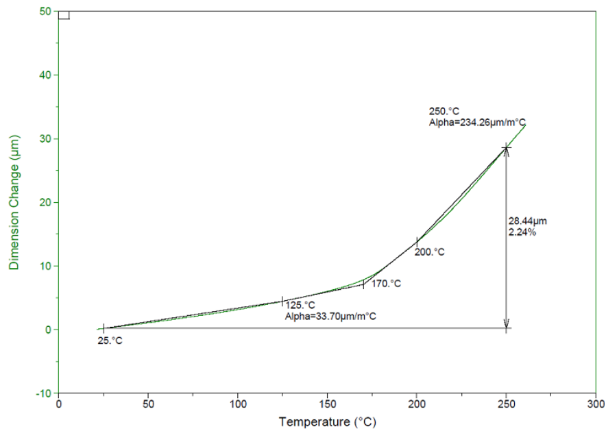
Figure 4 - CTE \alpha_1 and \alpha_2 by TMA
