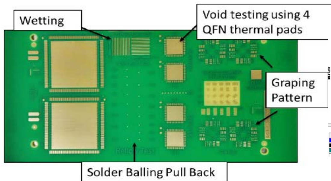
Fig 1 Picture of test board J with QFN thermal pads
