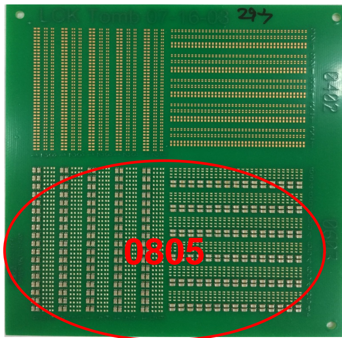
Figure 3 The Tomb solder beading test board (360 x 0805 component)
