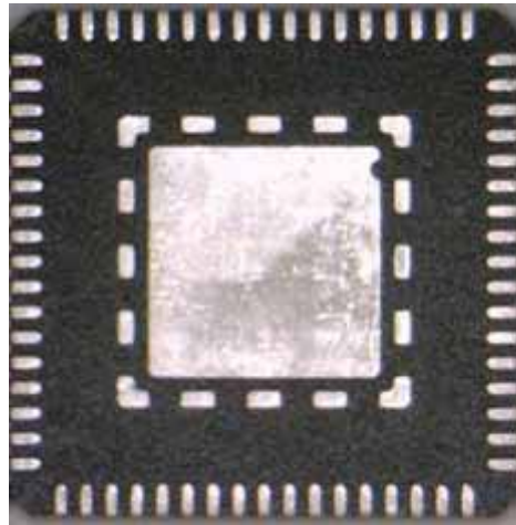
Figure 1. QFN component bottom view
