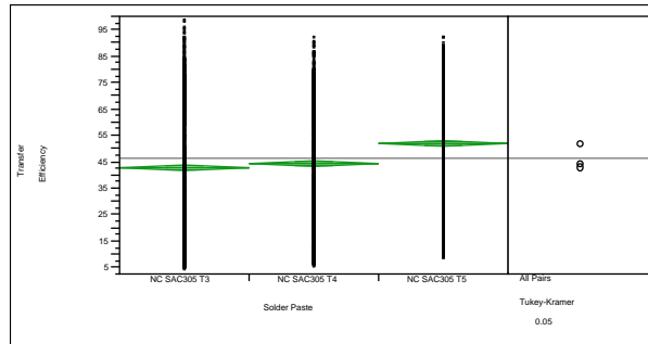
Figure 13 – Tukey-Kramer HSD by Solder Paste Type (Type 3, 4, 5) for Nano-Coated Stencils
