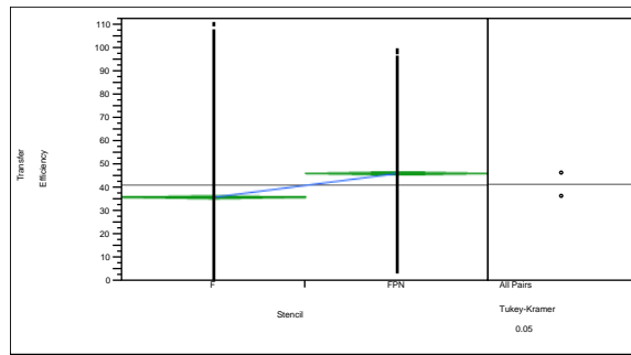
Figure 12 – Tukey-Kramer HSD by Stencil Type (Un-coated [F] versus Coated [FPN])
