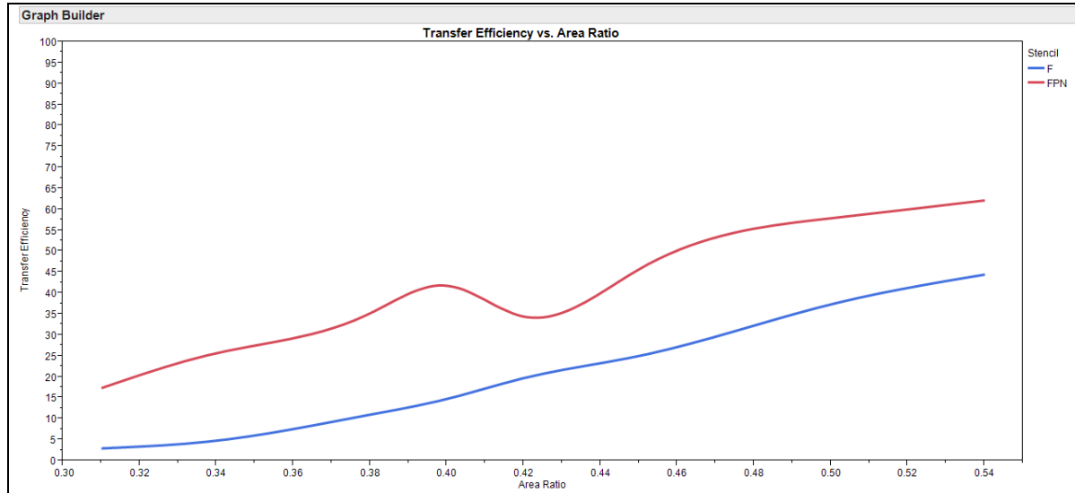
Figure 17 – 03015 Metric Uncoated (F) and Nano-coated (FPN) Stencils Mean TE% by Area Ratio for Both Stencil Thicknesses with Type 5 Solder Paste
