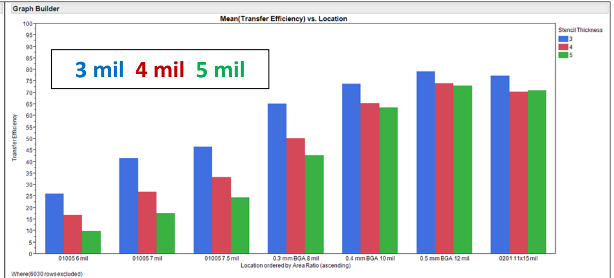
Polymer nano-coated stencils
