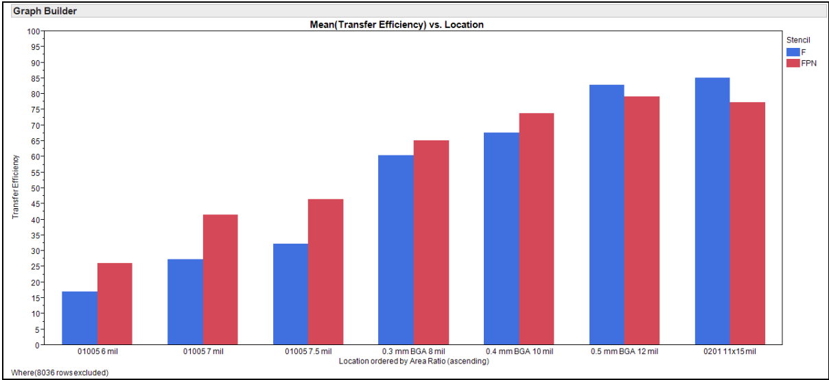
Figure 4 – Mean TE% by Location for 3 mil Thick Stencils (F-blue, FPN-red)
