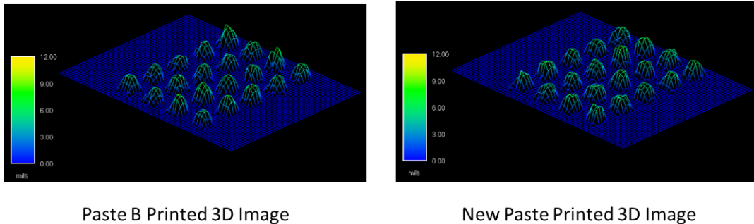
Figure 10 – Images of Solder Paste Bricks for Solder Paste B and New SP (50 mm/sec)
