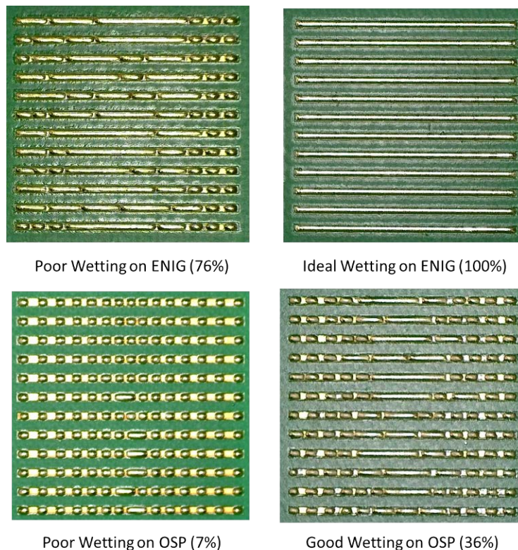
Figure 4 – F2A Wetting Pattern after Reflow for ENIG and OSP Finishes
