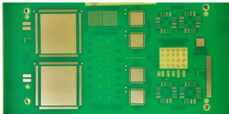
Figure 2 – F2A Reflow Test Circuit Board [5]
