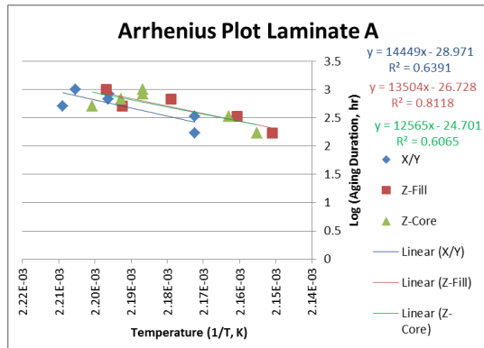
Figure 10a: Arrhenius Plots 1/Temperature (K) vs Log(Aging Duration, hr) for Laminate A; Calculated 50% EOL
