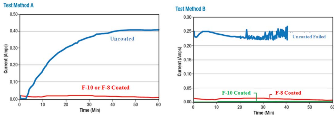
Figure 9: Potentiostat data showing current flow
