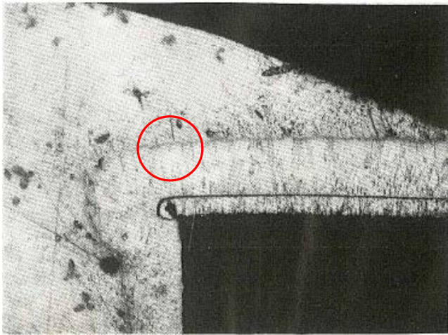
Copper burr pushed into hole
