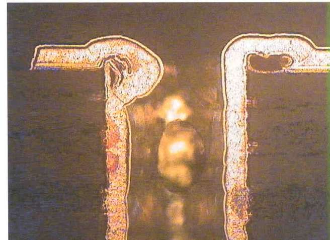
Copper plating void due to burr
