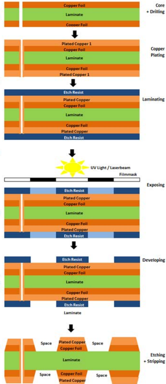
Figure 2: Panel plating
