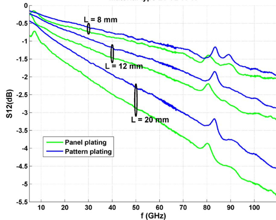
Material type B: CBCPW
