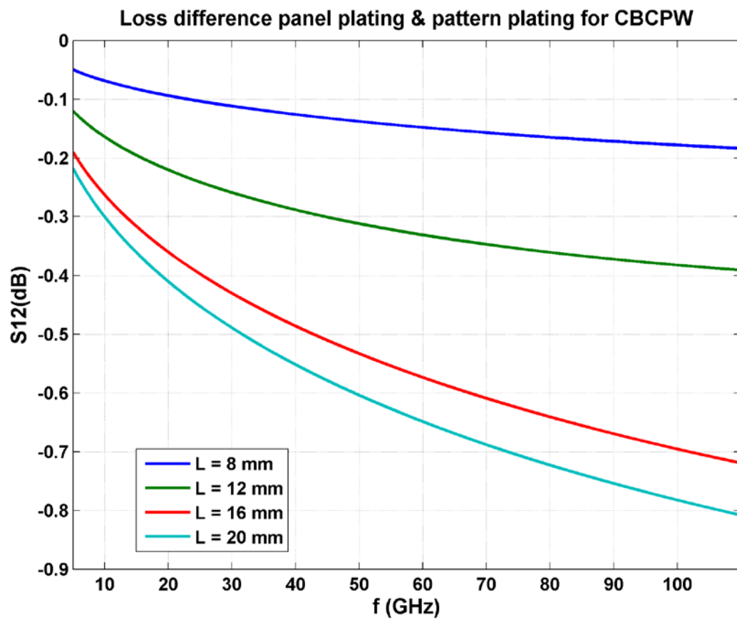
13: Loss difference CBCPW
