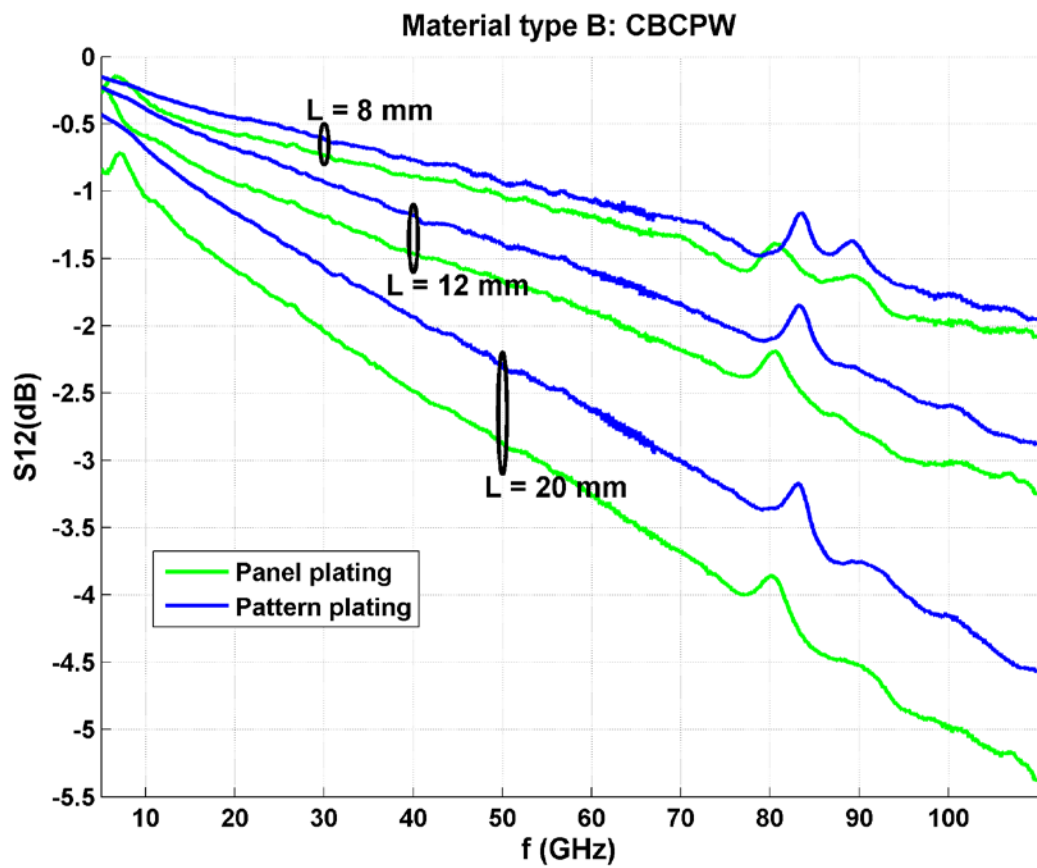
Figure 12: Material type B CBCPW
