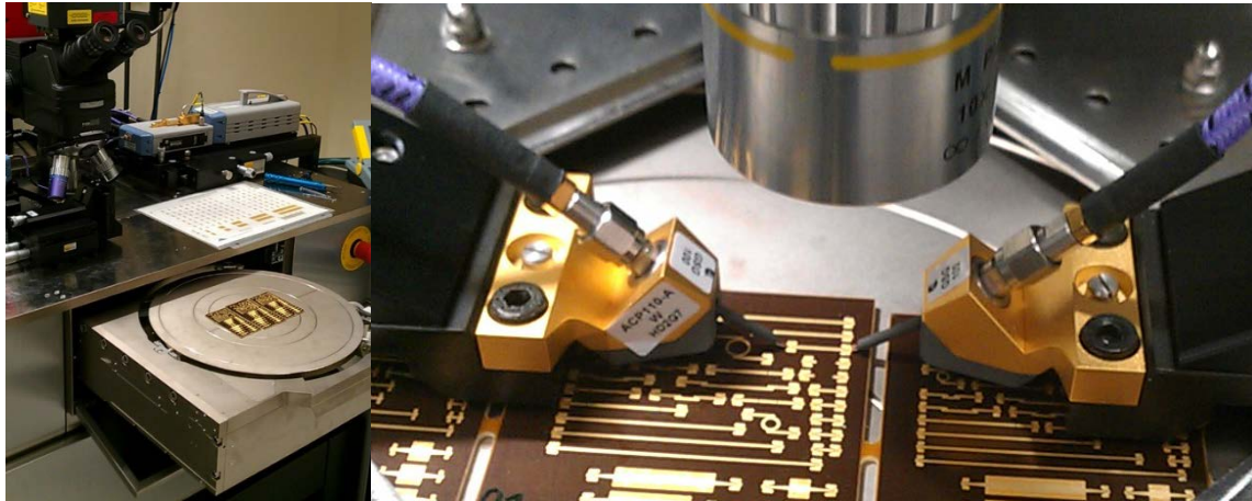
Figure 5: Measurement equipment
