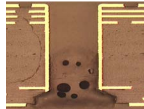
Back Drilled holes
