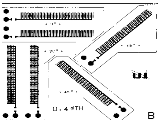
Figure 2 – CAF Test Vehicle
