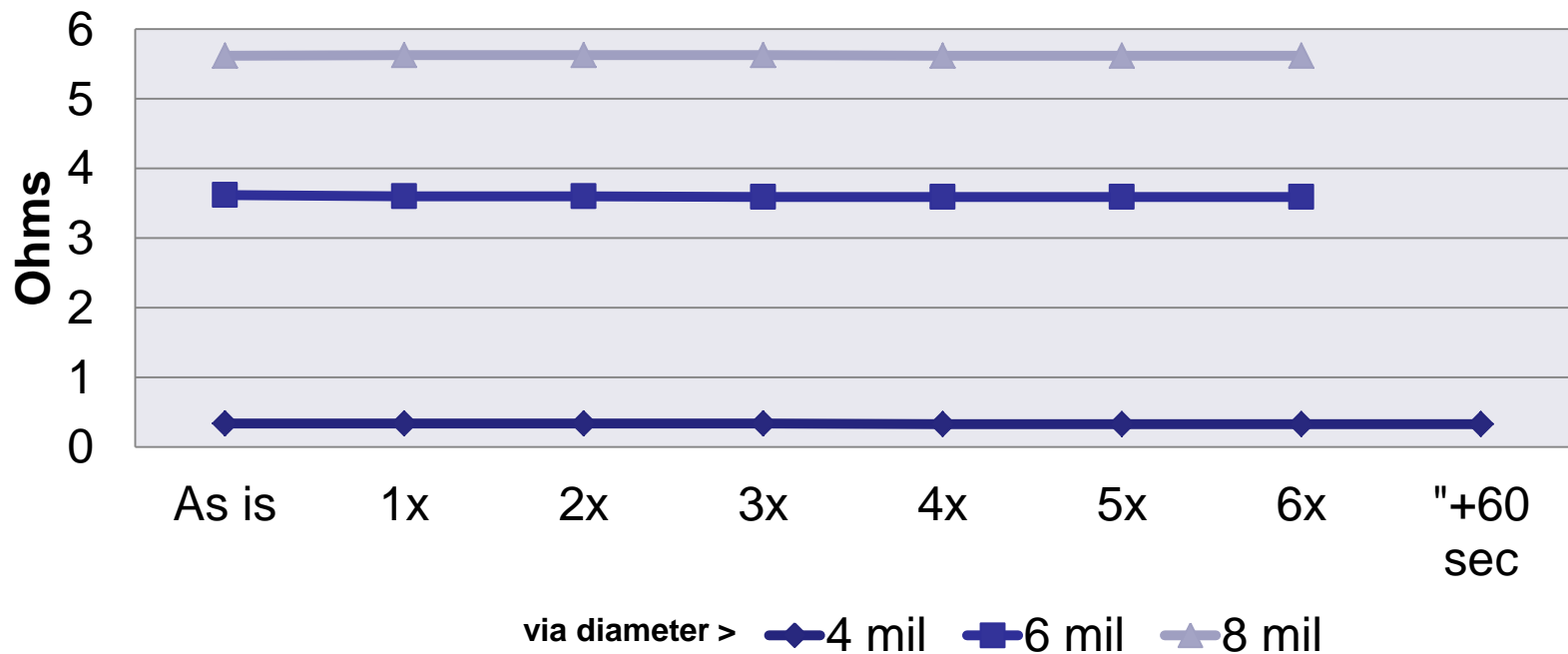
Daisy chain test vehicle of 120 paste vias Resistance change after 10 sec float @ 288° C
