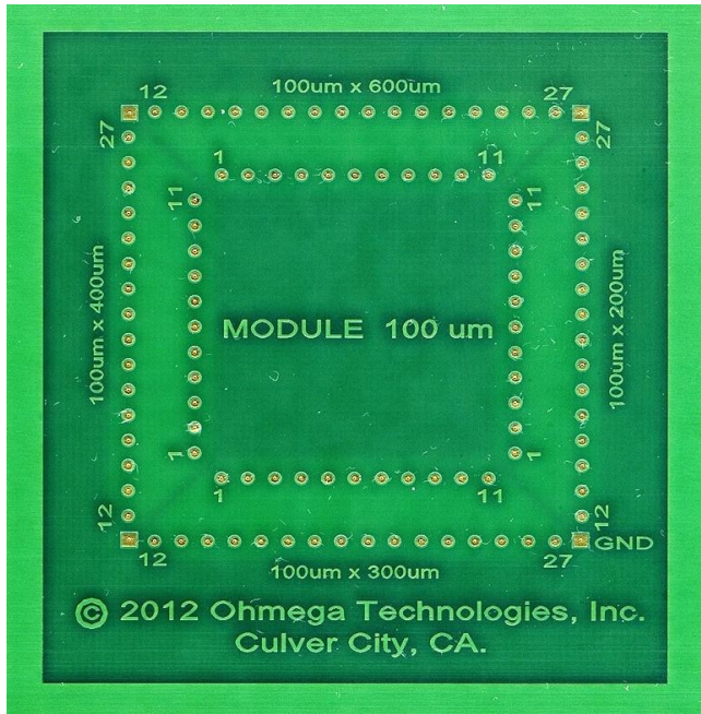
Figure 6 - multilayer board
