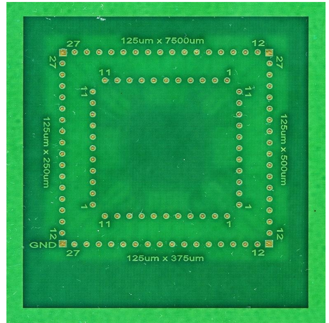
Figure 6 - multilayer board
