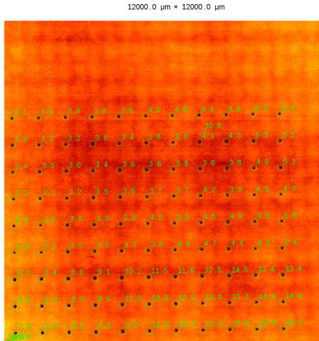
Evaluated BMV array with corresponding dimple
