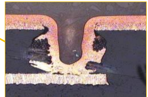
Glass fibre protrusion
