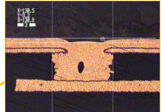
Copper foil over hang
