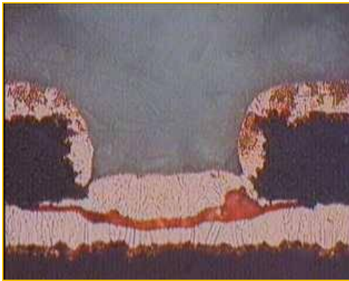
Wedge void at capture pad
