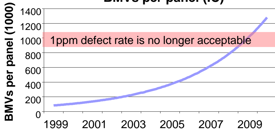
BMVs per panel (IC)
