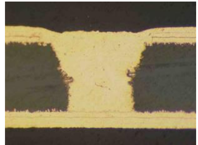
BMV diameter 80 \mu m Depth 77 \mu m with 12 \mu m Cu foil Plated Cu thickness 12 \mu m
