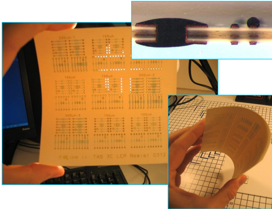
Same board but with another prepreg
