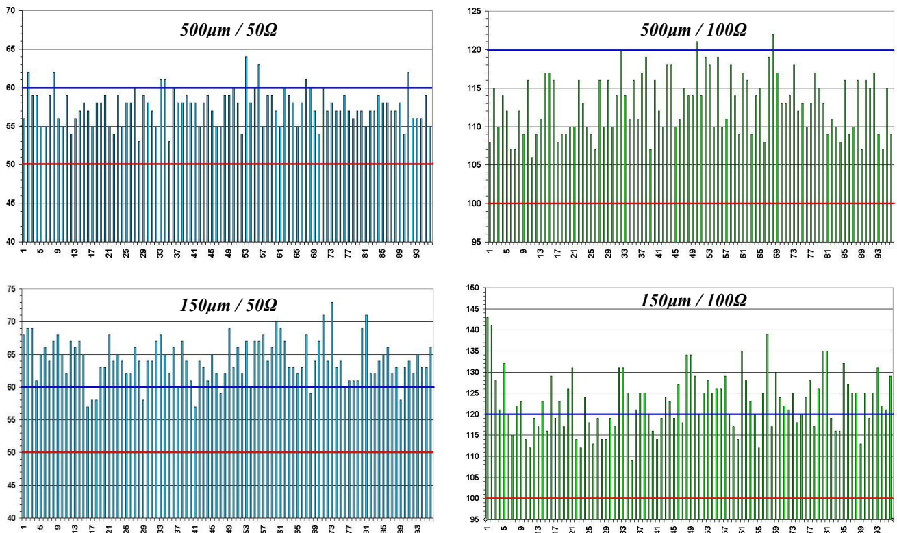
Figure 11 – Resistors values
