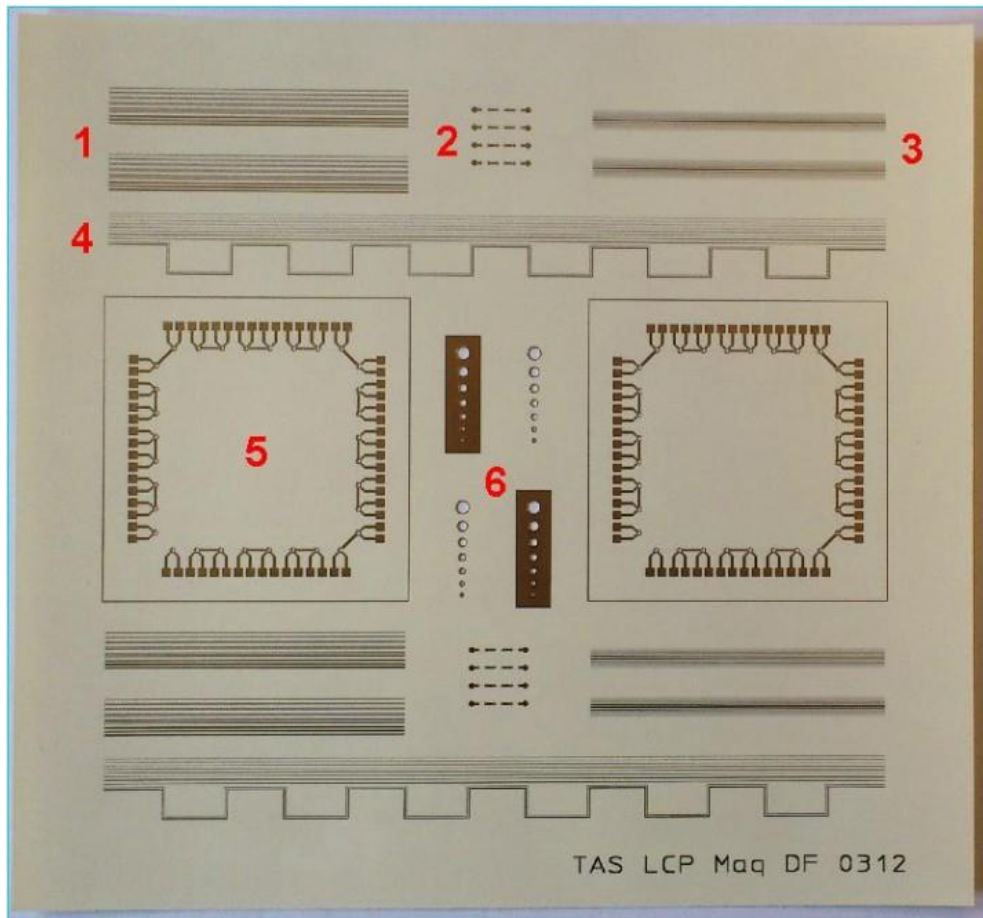
Double sided board on 100µm LCP
