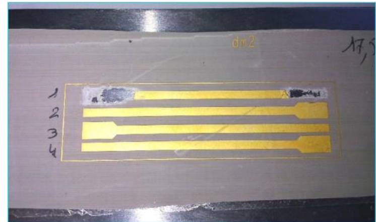
Peel strength test according to IPC
