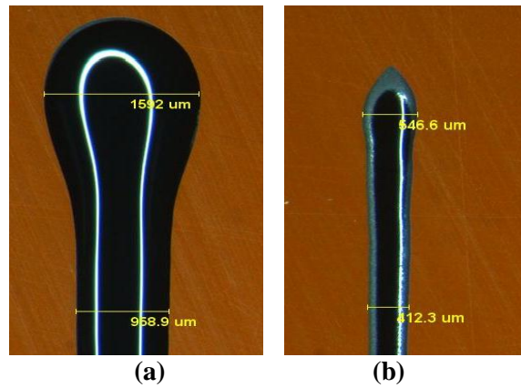
Figure 8 - (a) Uncontrolled material dispense (b) Controlled material dispense
