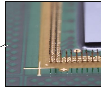
0.52mm contact height
