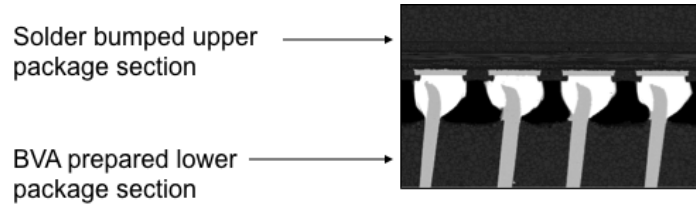
Figure 7. Cross section micrograph of BVA Cu wire tips protruding into the solder-bump contacts on the upper package section.
