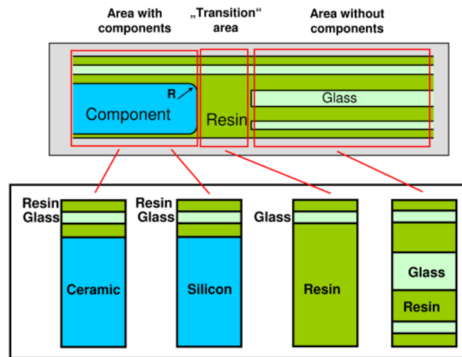
Figure 7: Simplified model of an embedded component in a printed circuit board
