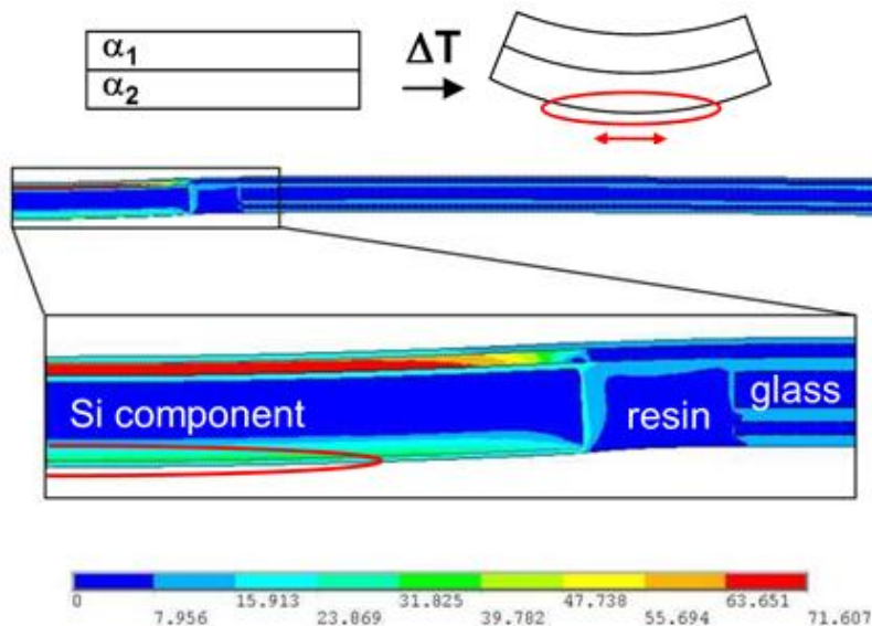
Embedded Si-chip
