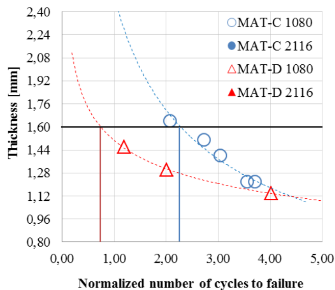
Figure 15: Normalized number of cycles to failure of QFN packages as a function of the PCB thickness
