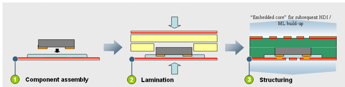
Figure 1 - Basic process flow for embedded components
