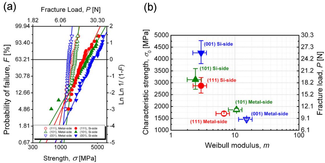
Figure 5a: B3B tests on Si-side and Metal-side Si chips Figure 5b: Characteristic strength vs. Weibull modulus diagram for the tested specimens.
