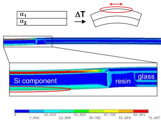
Figure 8: FEM-Simulation of embedded Si-chip
