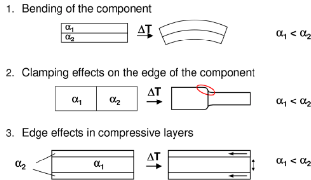
Figure 6: Cases of thermal stresses in a laminate
