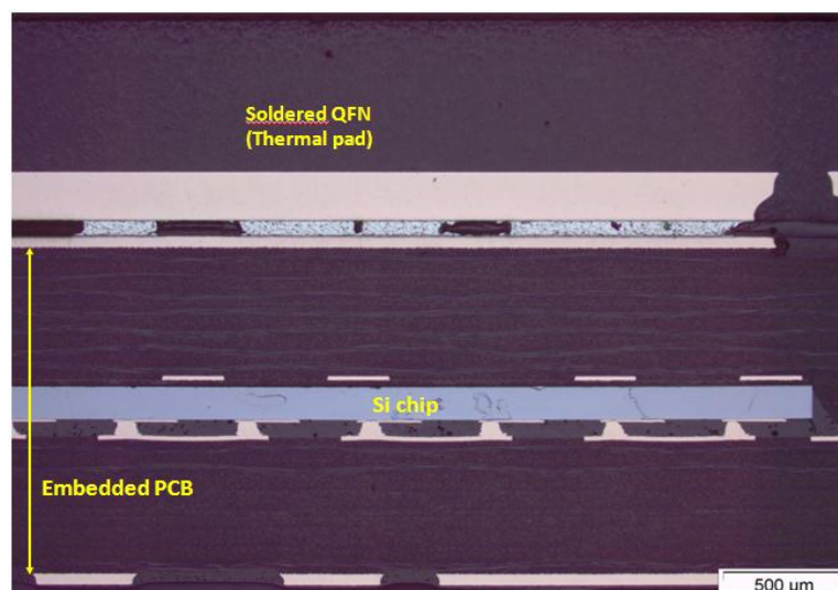
Figure 11 : Test vehicle cross-section view : soldered QFN overlapping an embeded Si chip
