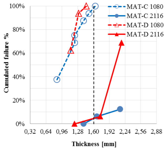
Figure 14: Cumulated failure of each population at the end of the test as a function of the PCB thickness
