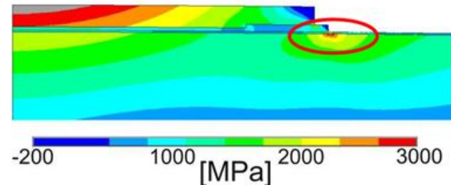
FEM simulation: B3B test
