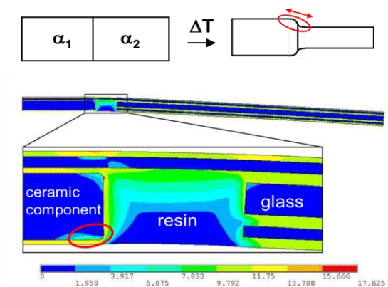
Figure 9: FEM-Simulation of embedded ceramic component
