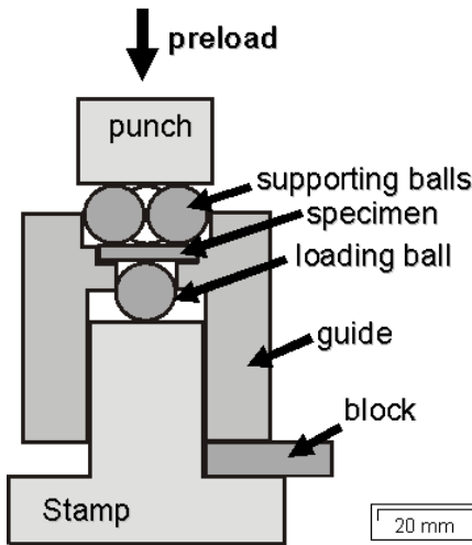
Figure 3: Schematic drawing of the B3B fixture
