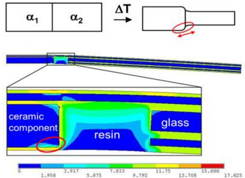
Embedded ceramic component
