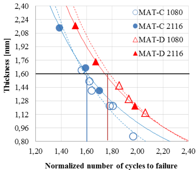
Figure 13: Normalized number of cycles to failure of BGA packages as a function of the PCB thickness
