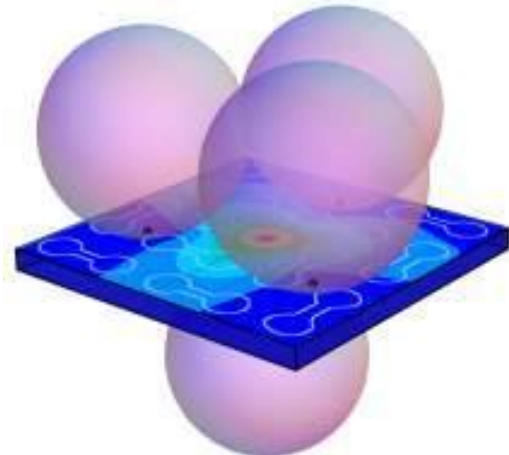
Figure 4: Stress field developed in the specimen during B3B testing, calculated with FEM.
