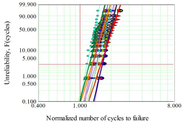
Figure 12: Weibull plot for 15 groups of BGA packages
