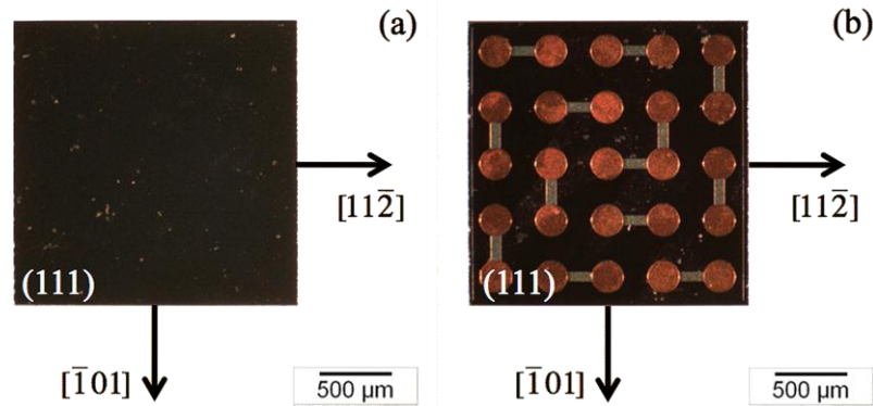
Figure 2: (a) Si-side and (b) metal-side with Cu-contacts (red) and Al-interconnects (white), crystallographic directions (as determined by EBSD) are explicitly indicated.
