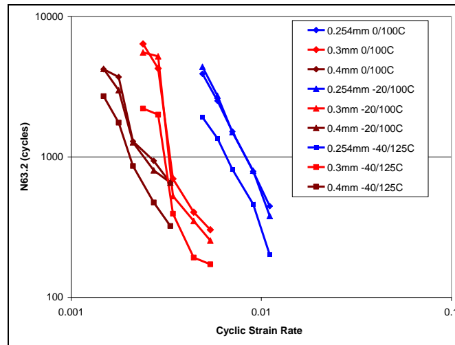
Figure 18. N63.2 versus Cyclic Strain Rate. Data is organized by solder ball diameter and accelerated thermal cycle condition.
