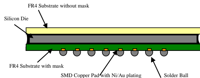
Figure 4. Cross- section of BGA design.
