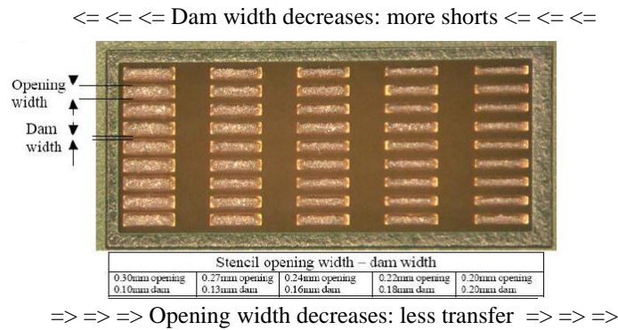
Figure 11. Printing pattern opening width and dam description
