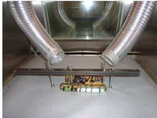
Figure 3. HALT Testing
