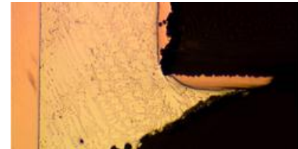
Copper dissolution and insufficient hole fill. Ref: Celestica 2007
