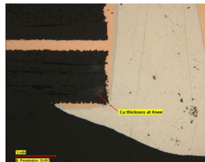
Figure 17. Baseline Process (100% Cu Dissolution at Knee)
