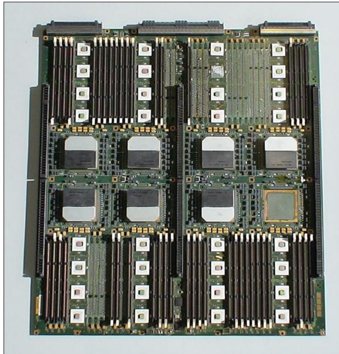
560 x 610mm (22" x 24"), 3mm (.120") thick PCB Board courtesy of IBM
