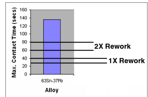
Process Window by Alloy (2)
