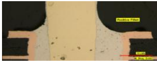
Figure 20: Positive Fillet from Rework Process
