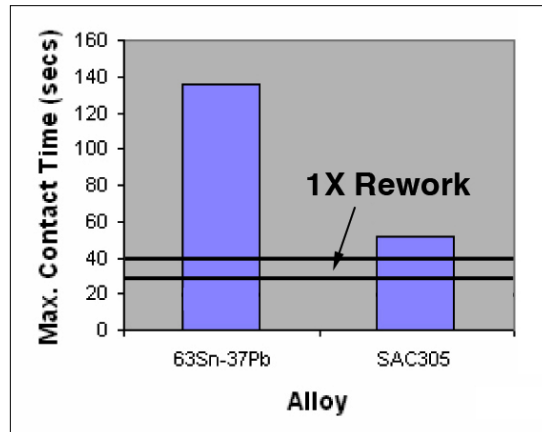
Process Window by Alloy (4)
