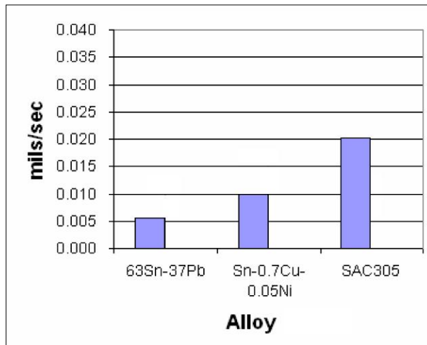
Dissolution Rates by Alloy (5)
