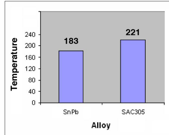
Melt temperature by alloy
