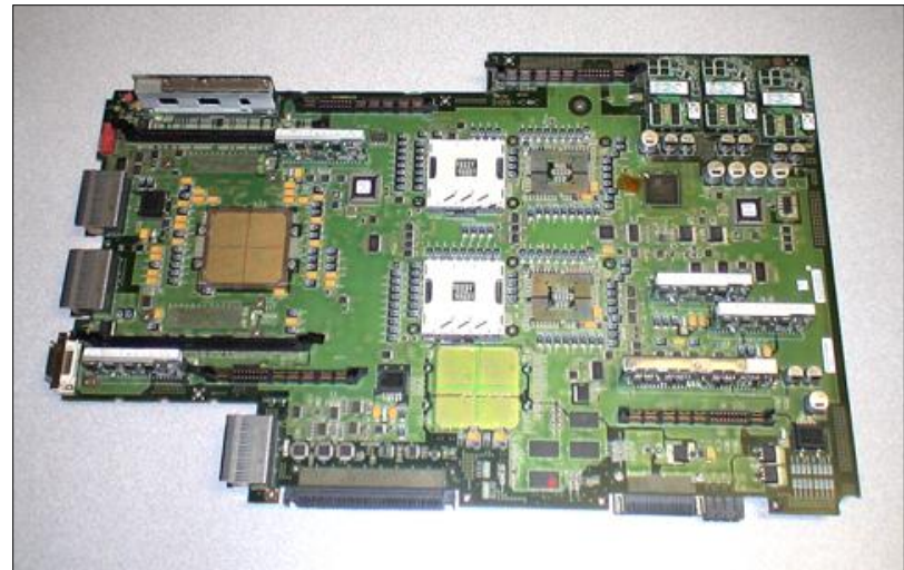
330 x 510mm (13" x 20"), 4mm (.160") thick PCB
