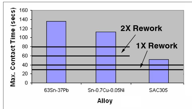
Process Window by Alloy (6)
