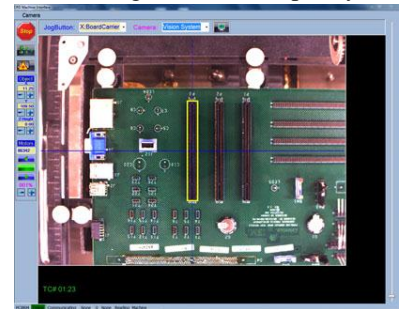
Figure 11: EZ-Line Alignment System
