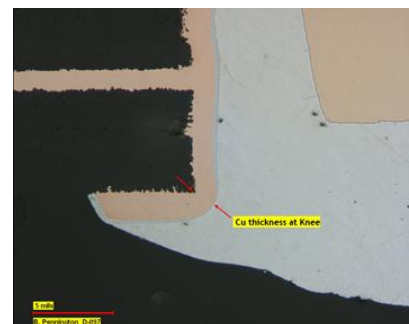
Figure 18. Alternate Process (Minimal Cu Dissolution at Knee)
