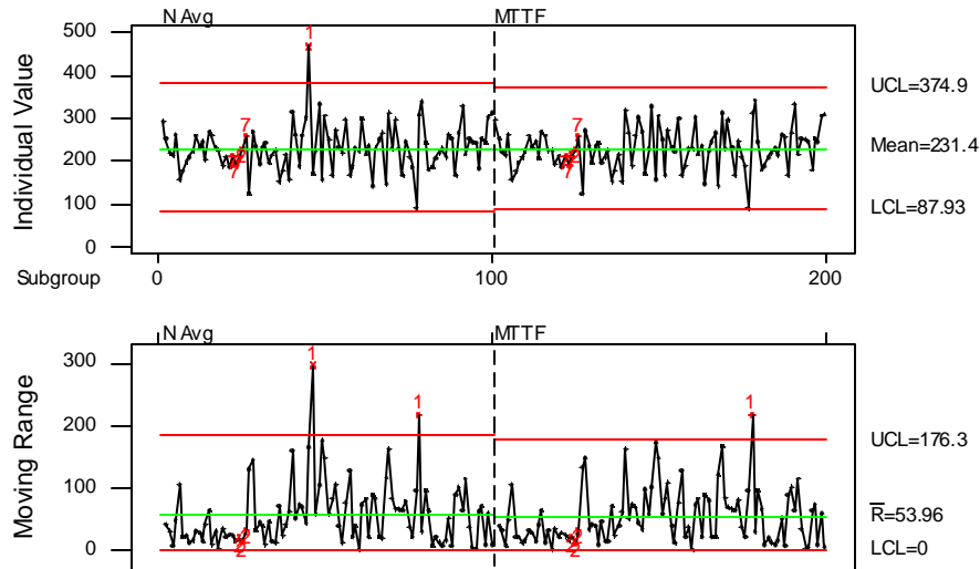
Figure 11 – Cycles to Failure Comparison
