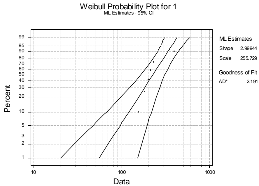
Figure 2 – Weibull Probability Plot, Sample 1
