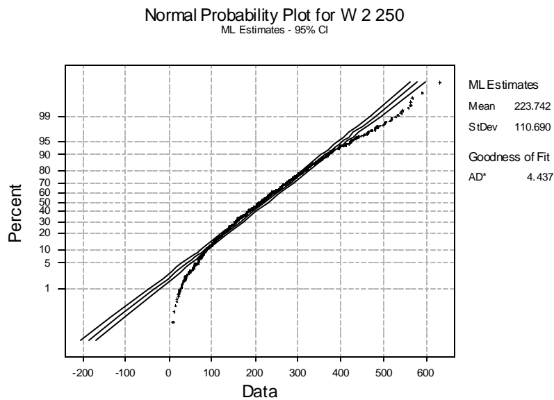
Figure 7 – Normal Fit to Weibull Simulation
