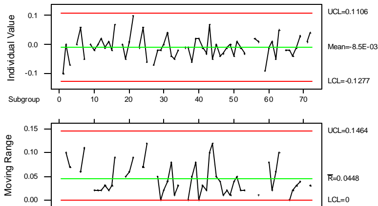
Figure 5 – Paired Differences, Clustered
