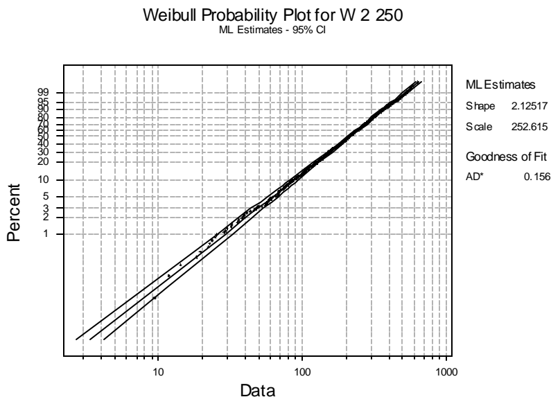
Figure 6 – Weibull Fit to Weibull Simulation
