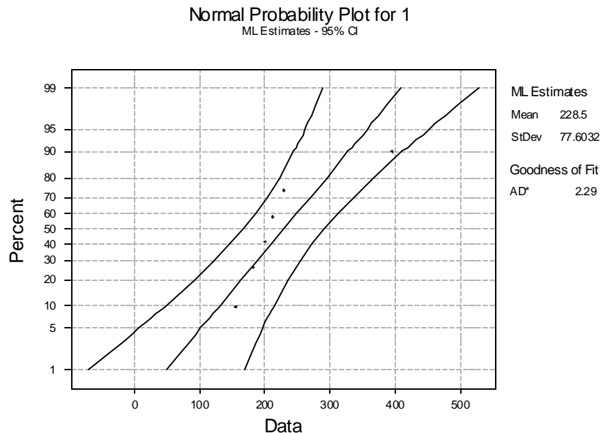
Figure 1 – Normal Probability Plot, Sample 1
