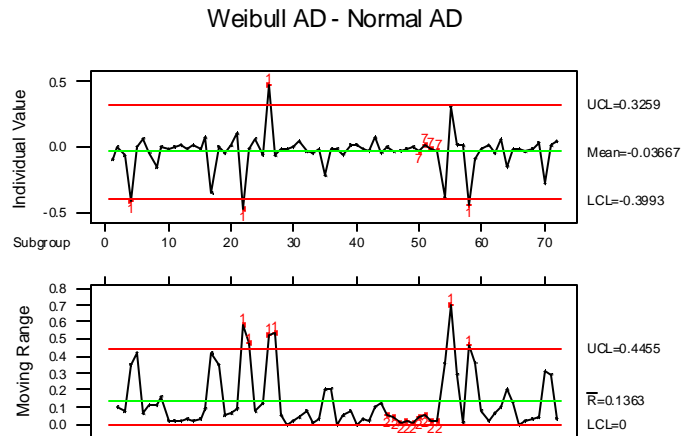
Figure 4 – Paired Differences
