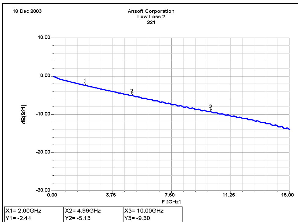
Figure 10 - FEA Transmission Line 16" Low Loss 2
