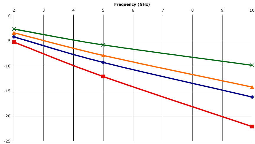
Figure 5 - Attenuation (Network Analyzer@ 2, 5, 10 GHz)
