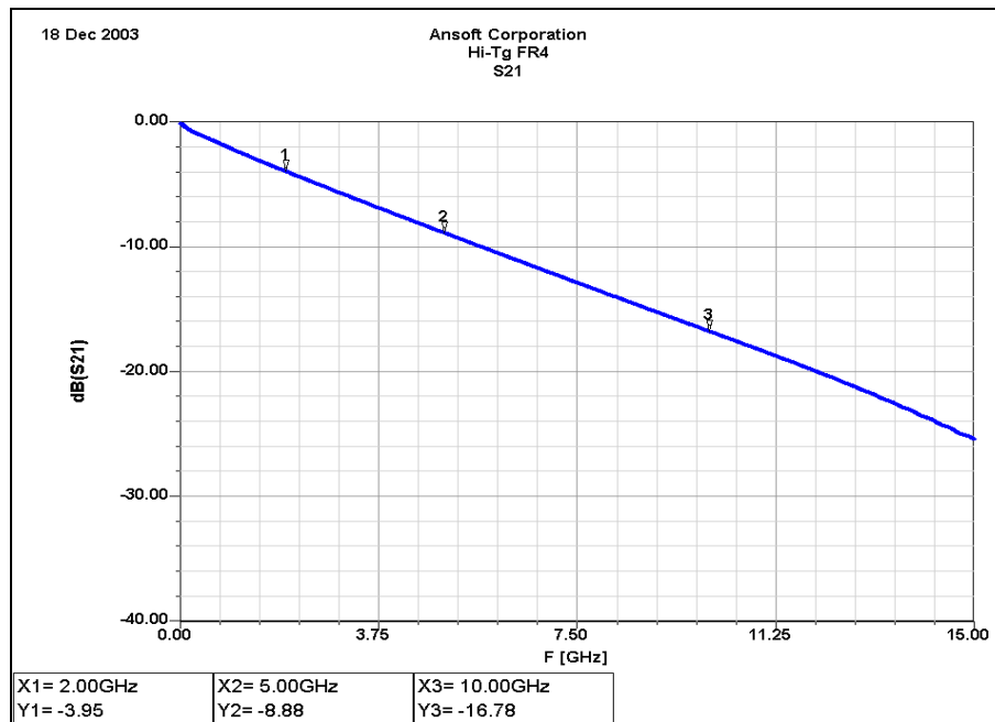
Figure 7 - FEA Transmission Line 16" Hi-Tg FR4
