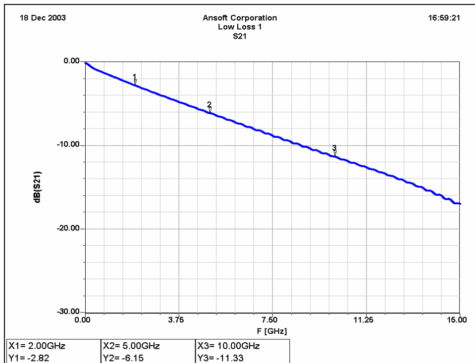
Figure 9 - FEA Transmission Line 16" Low Loss 1
