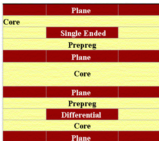
Figure 2 - Device under test (DUT) Stackup
