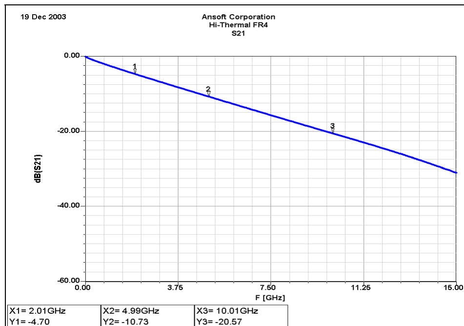
Figure 8 - FEA Transmission Line 16" Hi-ThermalFR4
