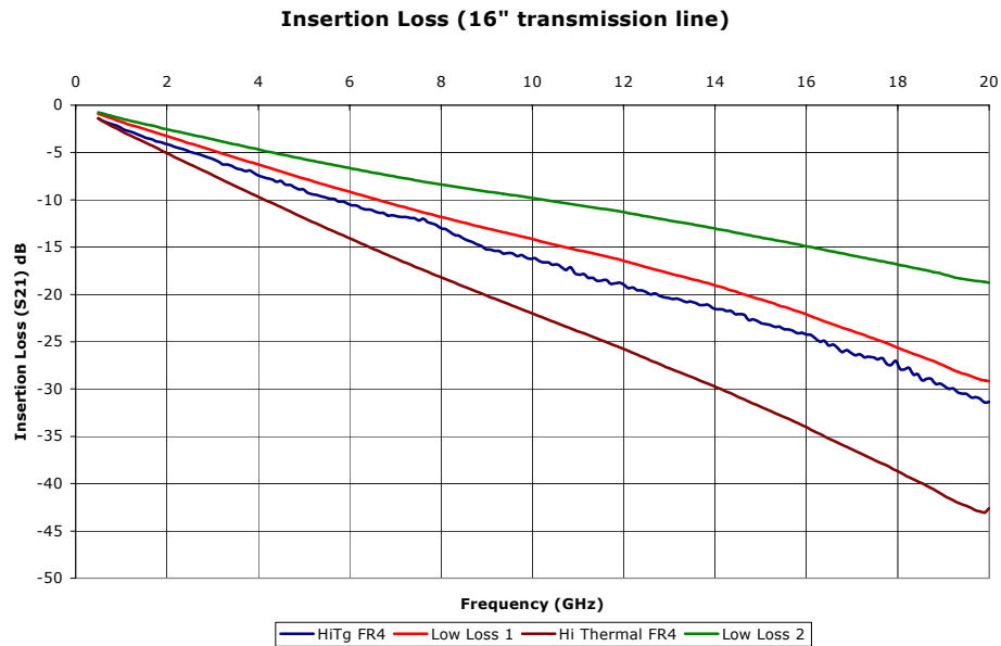
Figure 3 - Insertion Loss (attenuation)
