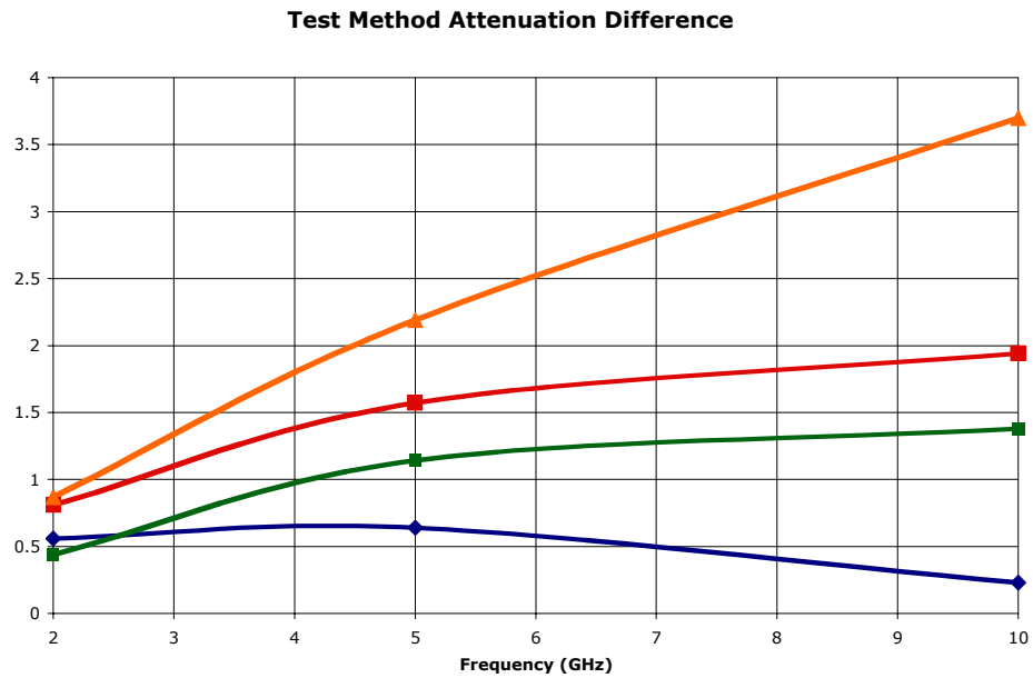
Figure 6 - Test Method Attenuation Difference
