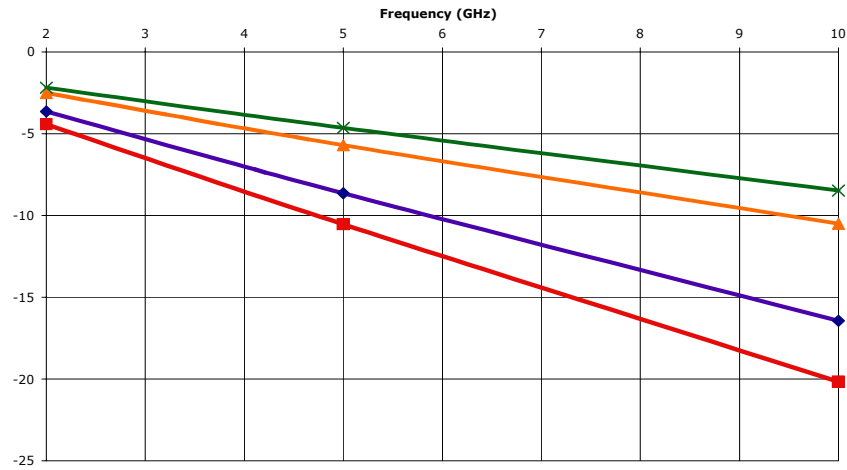
Figure 4 - Attenuation (dielectric+conductor loss)
