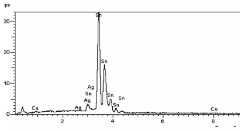
Figure 7b - Results in a Percentage [w/w] Distribution on the Surface of Sn94.6/ Ag4.4/Cu1.0
