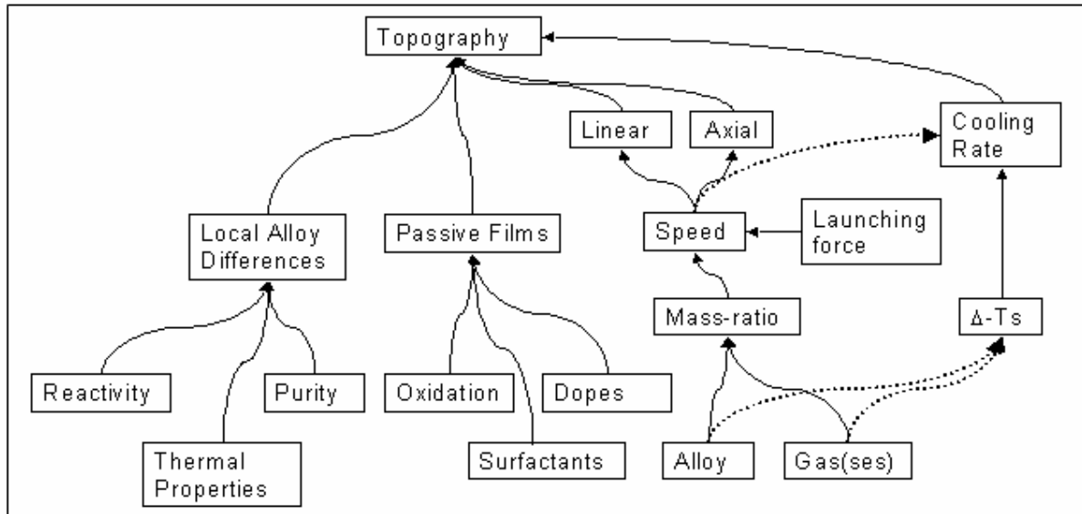
Figure 3 - A Map of Some of the Parameters Impacting The Topography of Solder Particles (DOES May Demonstrate Which Are the Most Significant)
