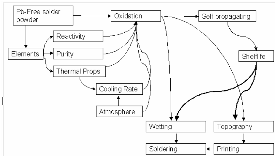
Figure 2 - A Mind Map Approach to the Interactions That Should Be Addressed When Designing For the Production of Pb-Free Soldering Paste
