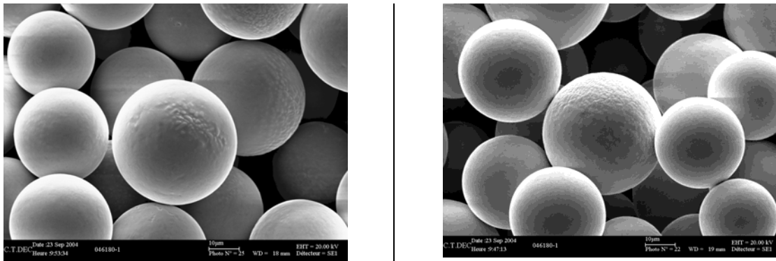
Figure 1a -b - SEM-Images of Class 3 Powder Produced from the Same Batch of SAC-Alloy. The Production of the Powder, However, Took Place Under Different Conditions. Depending on the Resolution of the Illustration, Qualitative Differences on the Surface Are Clearly Visible
