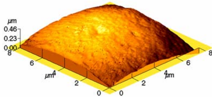
Figure 6 - A 3d-Image of a Surface of 64 \mu\text{m}^2 of A sn95.5/ag4.0/cu0.5 Solder Particle Generated by Atomic Force Microscopy (AFM). The Average Nano-Surface Roughness ( r_a ) Is 9.2 nm
