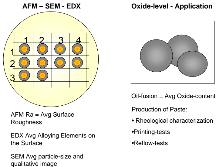
Figure 9 - This Shows the Different Tests Used In Phase 2 of This Project. They Will Result In Msa Compliant Detection Methods And Finally Will Lay The Foundation For Further Process Enhancements That Will Yield A Fully Iso-Ts-16949 Certifiable And Process Capable Pb-Free Solder Paste Manufacturing Process With Minimal Variation.
