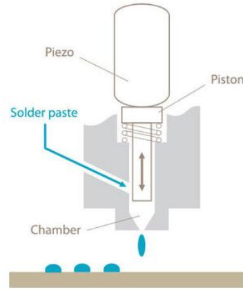
Figure 2 : A schematic of the jetting device used in the test.
